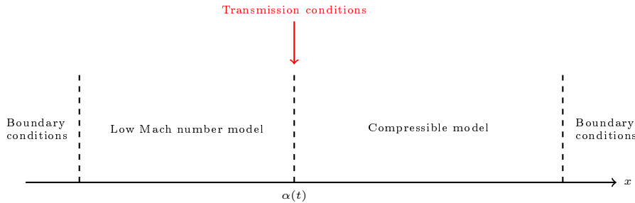
Figure 1: Coupling strategy
