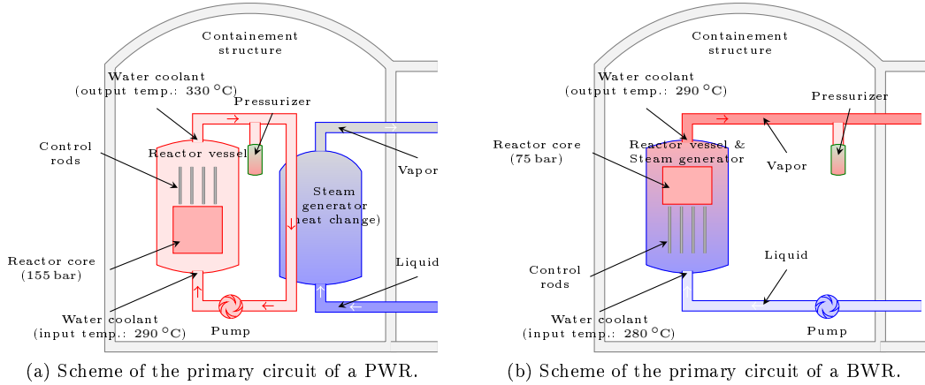
Figure 1: Scheme of nuclear reactors whose coolant is water: the major difference between PWR and BWR is the steam void formation in the core of the latter.
