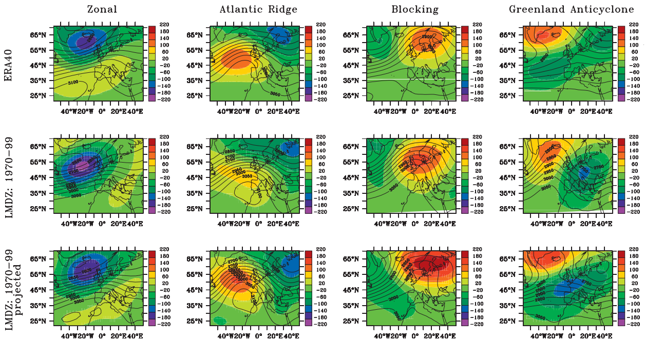
FIG. 1. The four weather regimes over the Europe–North Atlantic region obtained from 700-hPa daily geopotential height for (top) ERA-40 data obtained from the k -means algorithm, (middle) the LMDZ present-day climate simulation obtained from the k -means algorithm, and (bottom) the LMDZ present-day climate simulation obtained by projection on the ERA-40 regimes. The full fields (isolines) and regime anomalies (colors) are shown. Units are in geopotential meters.
