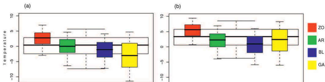
FIG. 4. Box-and-whisker plots of the daily mean temperature distribution ( ^{\circ}\text{C} ) in (a) 1970–99 and (b) 2070–99 over the region indicated by a rectangle in Figs. 2d,f. Wide white box represents the entire winter season distribution and colored boxes show the distributions inside the four weather regimes. The horizontal line within the box is the median; bottom and top box bounds show the 25th and 75th percentiles, respectively; bottom and top whisker bounds indicate the 5th and 95th percentiles, respectively. Color legend is as in Fig. 2.
