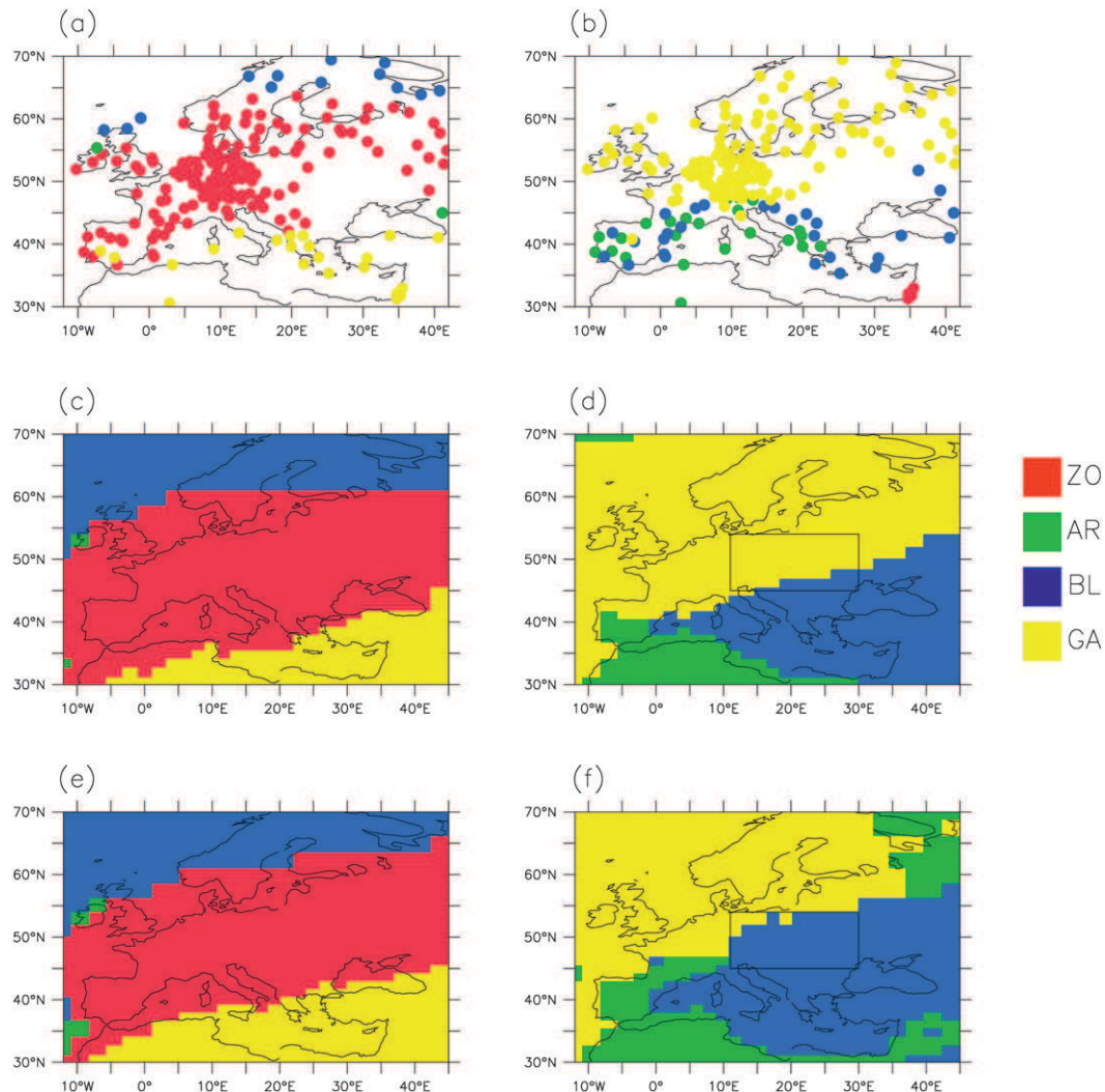
FIG. 2. Weather regimes favoring the occurrence of (a),(c),(e) warm and (b),(d),(f) cold temperatures over Europe: (a),(b) the observed relationship for the 1970–99 period, and the relationship simulated by LMDZ for (c),(d) the 1970–99 period and (e),(f) the 2070–99 period. Color legend: zonal regime (red), Atlantic Ridge (green), blocking (blue), and Greenland anticyclone (yellow).
