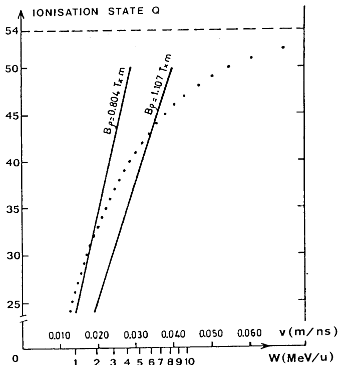
Fig.2. Most abundant charge for Xenon as a function of speed v , or energy W .
