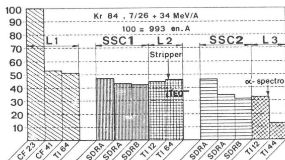
Fig.2 : Characteristics of a Kr beam :
