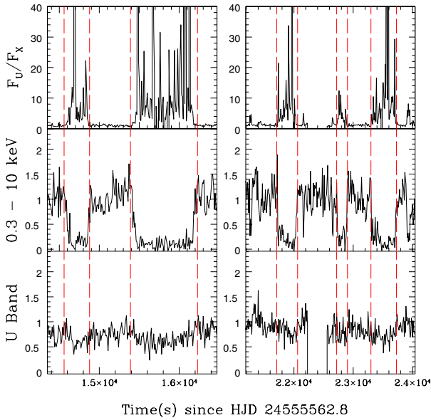
Fig. 6. Enlargement of the normalized light curves in 2011 showing the simultaneous occurrence of quiescent dips in the U band ( bottom panel ) and X-rays ( middle panel ) (0.3–10 keV) with a binning time of 10 s, together with the ratio of the U and X-ray band count rates ( top ). Vertical dashed (red) lines mark the dip start and end times.
