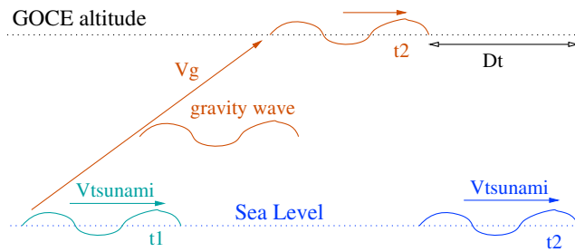
Figure 1. Scheme of tsunami and gravity wave propagation in the vertical plane along tsunami propagation direction (hereafter noted as x ). The time of the gravity wave excitation by the tsunami is t_1 . The time of gravity wave arrival at the GOCE altitude (after about 1 h) is t_2 . Tsunami position at this time is provided on the right of the figure. V_g stands for the gravity wave group velocity and Dt is the time delay between the arrival of the tsunami wave at the ocean surface and the arrival of the gravity wave above that point at the altitude of GOCE. Adapted from Occhipinti et al. [2013].
