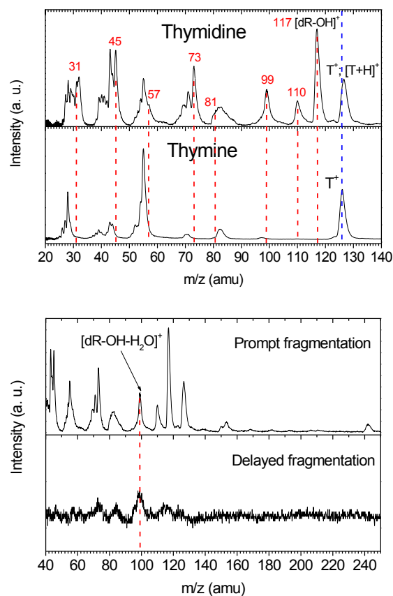
Fig. 2 (a): mass spectra of gas-phase thymidine (top) and thymine (bottom) after collision with 5 keV protons, in the thymine fragmentation region. The mass of cations corresponding to peaks appearing only in the thymidine spectrum are written in red, and the position of the thymine radical cation (126 amu) is indicated by blue dashes. (b): mass spectra of thymidine fragment cations formed by prompt dissociation (ns timescale; top) and undergoing delayed fragmentation ( \mu s timescale; bottom).
