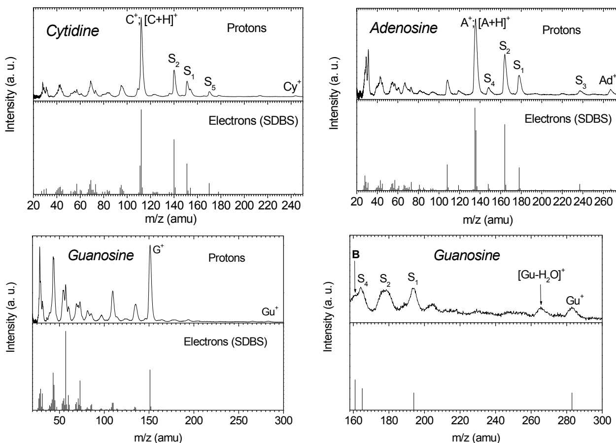
Fig. 3 Mass spectra of gas-phase (a) cytidine, (b) adenosine and (c) guanosine after collision with 5 keV protons (top) and low-energy electrons (bottom, from the SDBS database). Cytidine, cytosine and protonated cytosine cations are denoted Cy + , C + and [C + H] + , respectively. Adenosine, adenine and protonated adenine cations are denoted Ad + , A + and [A + H] + , respectively. Guanosine and guanine radical cations are denoted Gu + and G + , respectively. (d) is a magnification of (c), to allow fragments heavier than the base to be clearly seen. Their notation follows that of Fig. 4.
