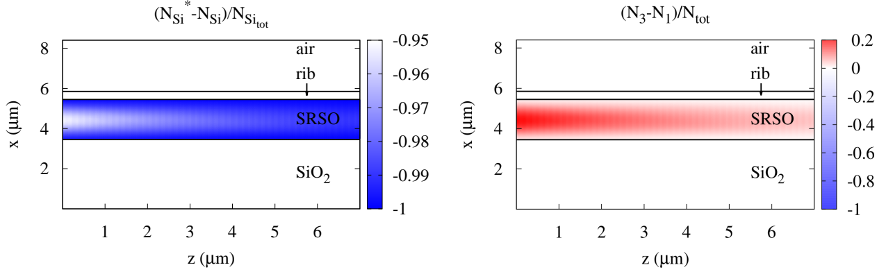
FIGURE 10. Relative population differences along the direction of propagation of Si-ng (on the left) and for the neodymium ions (on the right) in \text{SiO}_x :Si-ng :Nd ^{3+} system for a pump power equal to 1000 \text{ mW} \cdot \text{mm}^{-2}
