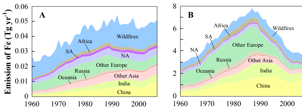
Figure 4. Temporal trends of Fe emissions of fine ( PM_1 ) (a) and medium-to-coarse ( PM_{1-10} and PM_{>10} ) (b) particles from combustion sources from 1960 to 2007. Fe emissions from wildfires are shown separately with energy-related activities separated by region (NA for North America and SA for South America).
