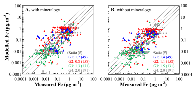
Figure 14. Plots of modelled and measured Fe concentrations attached to aerosols in surface air. The Fe content of dust was calculated from the new mineralogical data (a) or prescribed as 3.5% (b). All stations were divided into four groups based on the relative differences between (a) and (b): G1, difference \geq 30\% (blue triangles); G2, 20\% \leq difference < 30\% (red triangles); G3: 10\% \leq difference < 20\% (green triangles); G4, difference < 10\% (grey squares). The ratios between measured and modelled concentrations as geometric means are listed with the number of stations in parentheses for each group.
