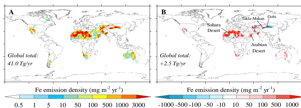
Figure 5. Average Fe emission from dust sources for 2000–2011 using the new mineralogical data set (a) and the difference of average Fe emission from dust sources for 2000–2011 using the new mineralogical data set relative to that using a constant Fe content (3.5%) (b). A positive value in (b) indicates a larger emission density by using the new mineralogical data set.
