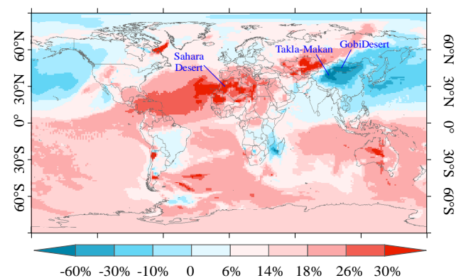
Figure 13. Relative differences in simulated Fe concentrations attached to aerosols in surface air when using the new mineralogical data and prescribing a constant Fe content in dust (3.5%). A positive difference indicates a higher Fe concentration when using the new mineralogical data.
