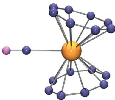
Fig. 5 Crystal structure of the anion [U(Cot)_2(CN)]^- .
