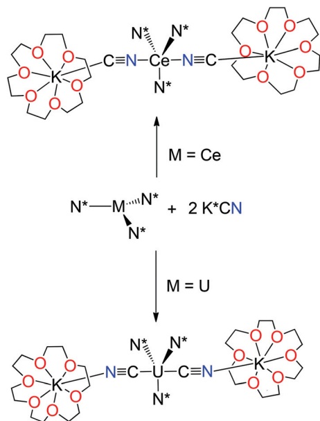
Scheme 6 Cyanide linkage isomerism in the anions [MN^*_3(CN)_2]^{2-} ( M = \text{Ce, U} ).
