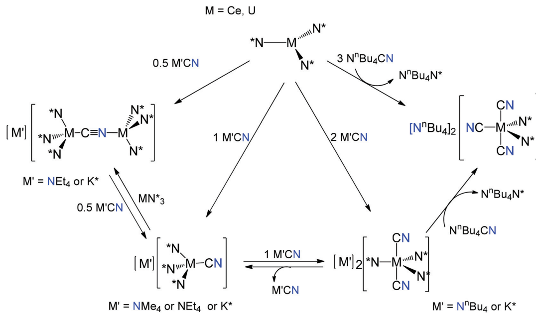
Scheme 5 Syntheses of uranium(III) cyanide complexes in the [\text{MN}^*_3] series.
