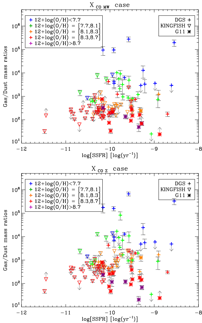
Fig. B.1. G/D as a function of SSFR for the 2 values of X_{\text{CO}} : X_{\text{CO}, \text{MW}} (top) and X_{\text{CO}, z} (bottom). The colours code for the metallicity of the galaxies and the symbols differentiate between the three samples: DGS (crosses), KINGFISH (downward triangles) and G11 (stars).
