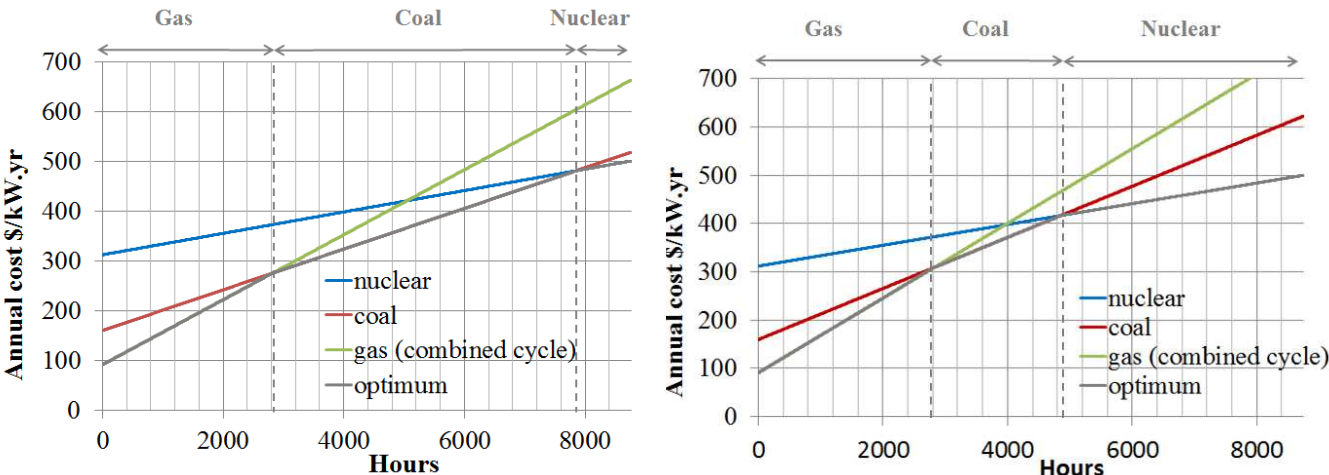
Figure 3: Screening curve example (cost data from Salvadores and Kepler (2010)), 8% discount rate, no carbon price (left figure) and $30/tonCO 2 (right figure)
