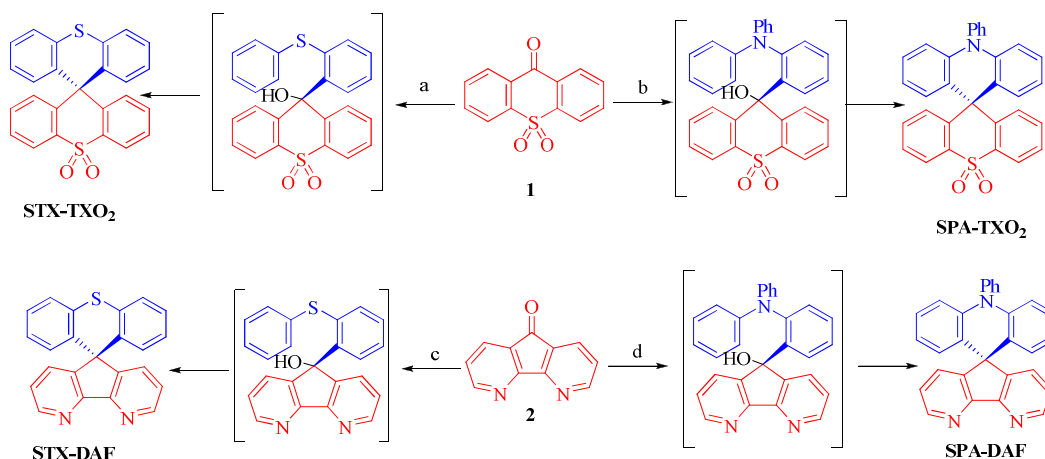
Scheme 2 : Synthesis of STX-TXO 2 , SPA-TXO 2 , STX-DAF and SPA-DAF
