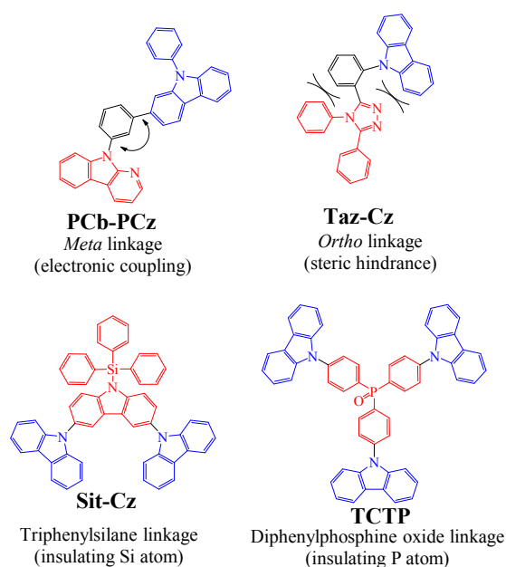
Chart 1. Different design strategies for \pi -conjugation disruption
