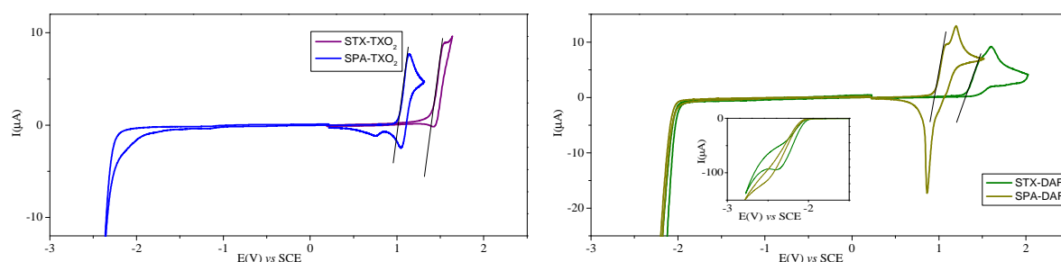
Figure 4. Cyclic voltammetry (100 mV/s) in \text{CH}_2\text{Cl}_2 /[ \text{Bu}_4\text{N} ][ \text{PF}_6 ] 0.2 M of STX-TXO 2 (violet line) and SPA-TXO 2 (blue line) (left) and of STX-DAF (green line), and SPA-DAF (yellow green line) (right).
