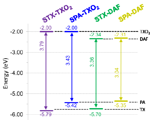
Figure 5. HOMO/LUMO energy levels and \Delta E_{\text{el}} (eV) obtained from electrochemical investigations
