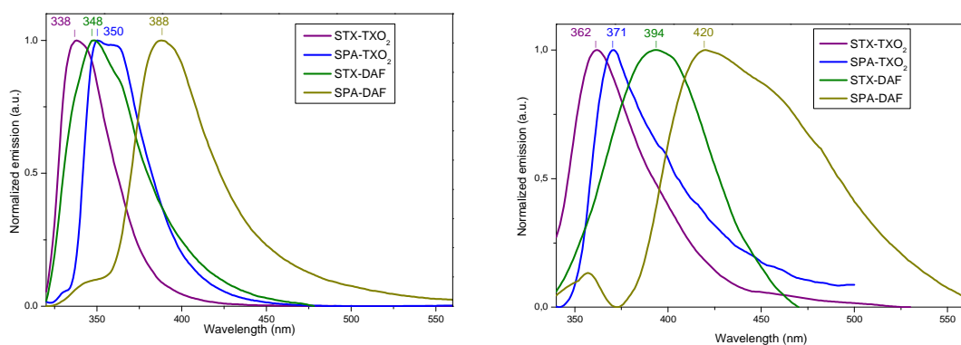
Figure 8. Emission spectra of the four dyes in cyclohexane (left) (concentration \sim 10^{-3} M) and in the solid state (thin film, deposited on a sapphire plate from 50 \mu L of a 10 g/L solution) (right).
