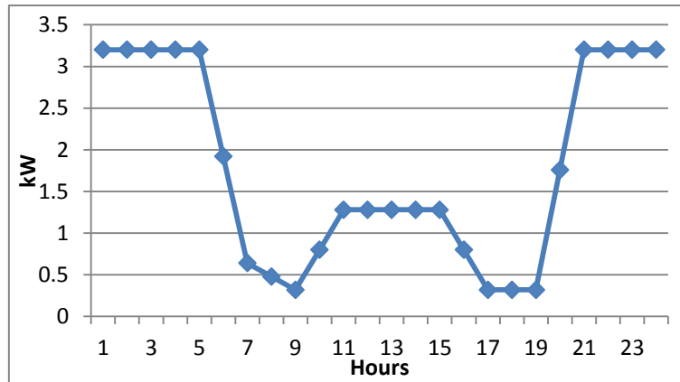
Figure 3: Hypotheses of power connected to the grid for an average vehicle
