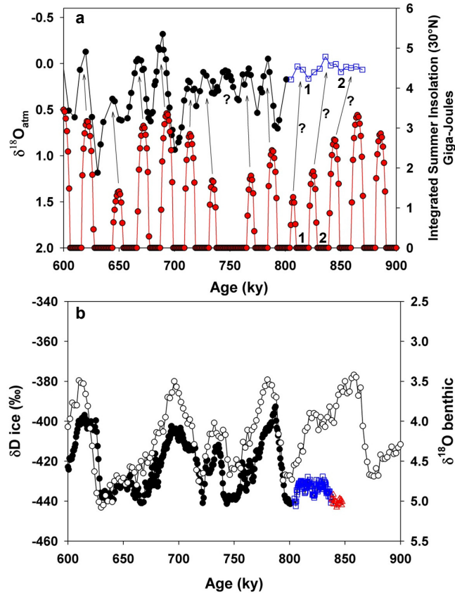
Figure 9. Attempting to reconstruct the timescale for the basal ice sequence: (a) zoom on the \delta^{18}\text{O}_{\text{atm}} curve vs. integrated summer insolation at 30° N (see Fig. 1e) and (b) comparison of the benthic \delta^{18}\text{O} curve (open circles) to the EPICA \delta\text{D}_{\text{ice}} profile (black dots), where the basal ice timescale was linearly “compressed” using tie points 1 and 2 in (a) (see text for details).
