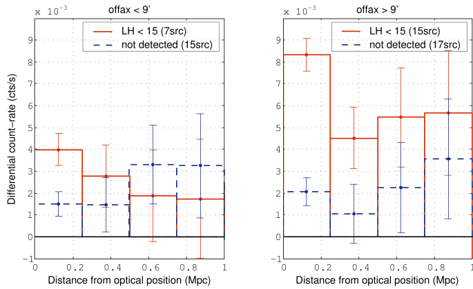
Fig. 12. Stacking analysis of the redMaPPer clusters not associated with any X-ray detection or coinciding with a marginal source (detection_likelihood <math>< 15</math>). Left panel: redMaPPer positions located at an off-axis radius <math>< 9'</math>. Right panel: redMaPPer off-axis positions between 9–12'.
