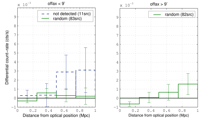
Fig. 13. Stacking analysis around random positions, not associated with any X-ray detection within 1 arcmin. Left panel: offaxis <math>< 9'</math>, Right panel: offaxis >math>9'</math>. Overlaid on the left panel is the signal obtained when removing four redMaPPer positions not associated with any detected source but for which some intensity enhancement is conspicuous on the X-ray pixel images.
