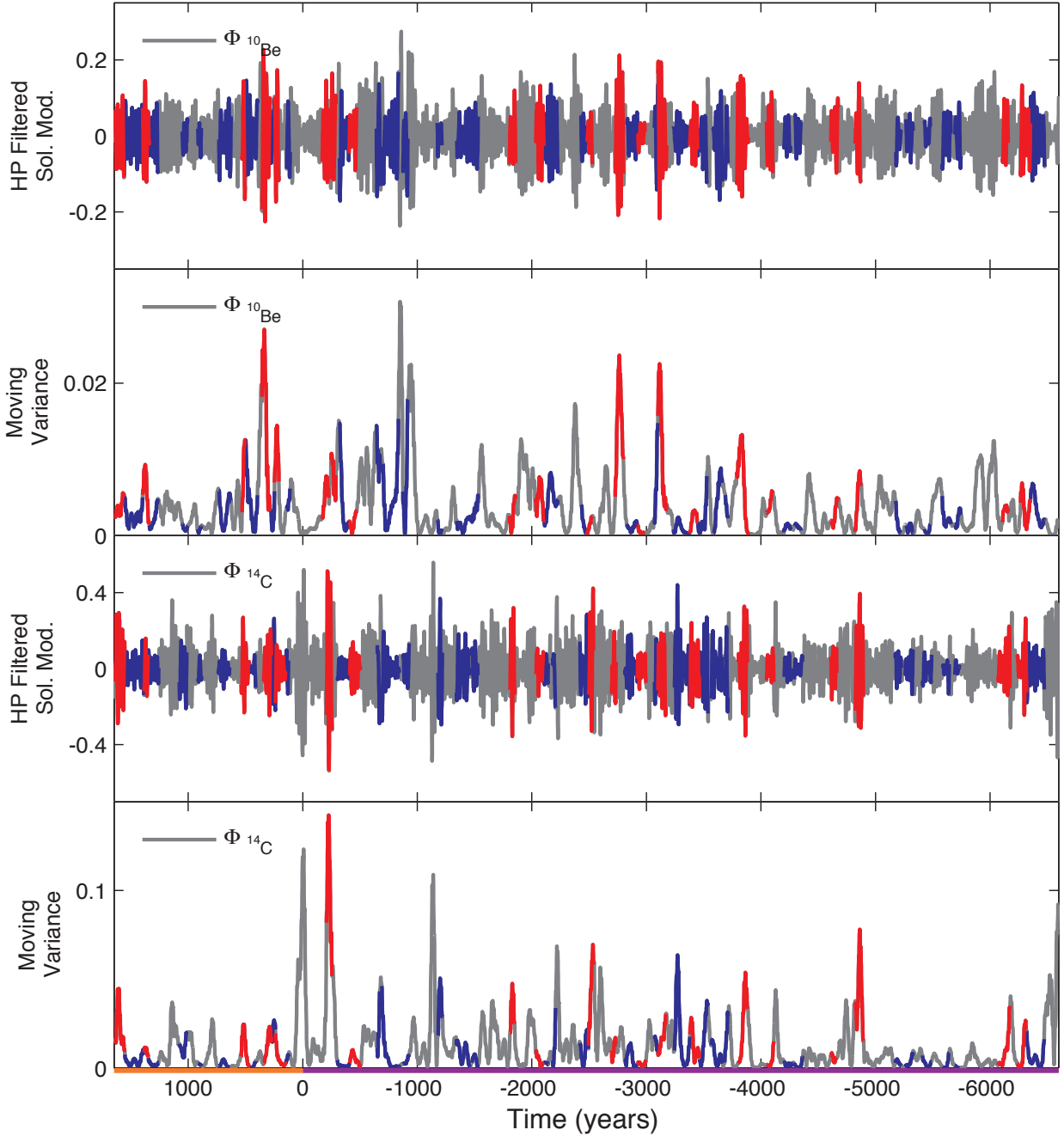
Fig. 7. Temporal changes in high-pass filtered \Phi_{10\text{Be}} and \Phi_{14\text{C}} ( first and third rows , respectively) with a cutoff frequency of (1/30) \text{ year}^{-1} . Blue and red lines show identified grand minima and maxima, respectively. The second and forth panels show the moving variance of high-pass filtered \Phi_{10\text{Be}} and \Phi_{14\text{C}} . The orange and purple colors show the dates AD and BC, respectively.
