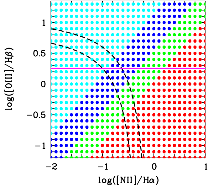
Fig. A.1. [\text{O III}] \lambda 5007/\text{H}\beta vs. [\text{N II}] \lambda 6584/\text{H}\alpha diagram with a grid color-coded like in the legend of Fig. 4 according to metallicity. Virtually all galaxies on the star-forming sequence (between the black dashed lines) and above the magenta line (i.e., with [\text{O III}] \lambda 5007/\text{H}\beta > 1.8 ) have \text{O}/\text{H} < 8.6 on the KD02 metallicity scale (cyan symbols).
