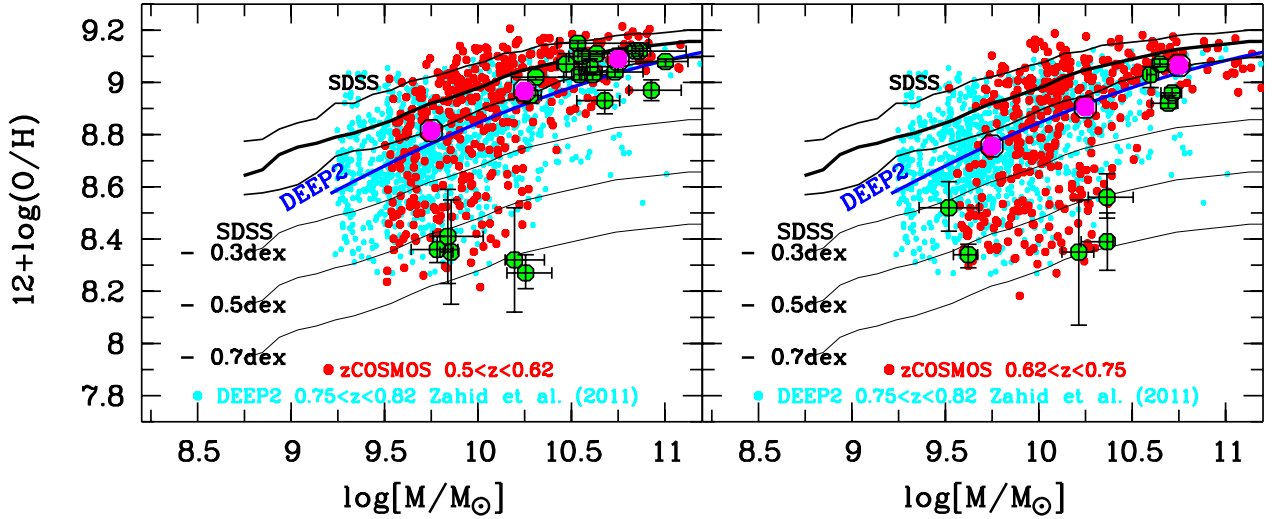
Fig. 5. MZR of zCOSMOS ELOX 0.5 < z < 0.75 galaxies (red circles) and galaxies with O/H measurements based on additional ISAAC spectroscopy (green filled circles), compared to the local MZR of Tremonti et al. (2004) and the MZR at 0.75 < z < 0.82 found by Zahid et al. (2011) using the DEEP2 sample. The individual DEEP2 data are shown as cyan symbols, while the mean DEEP2 MZR from Eq. (8) in Zahid et al. (2011), converted to the KD02 calibration, is shown as a blue line. The mean O/H values of zCOSMOS galaxies in three mass bins are shown as large magenta filled circles. While both zCOSMOS and DEEP2 galaxies at z \sim 0.5-0.8 have similar (slightly lower) metallicities at the higher masses compared to z \sim 0 , a population of galaxies with metallicities lower by a factor 2–3 than SDSS exists at the lowest masses probed by zCOSMOS and DEEP2.
