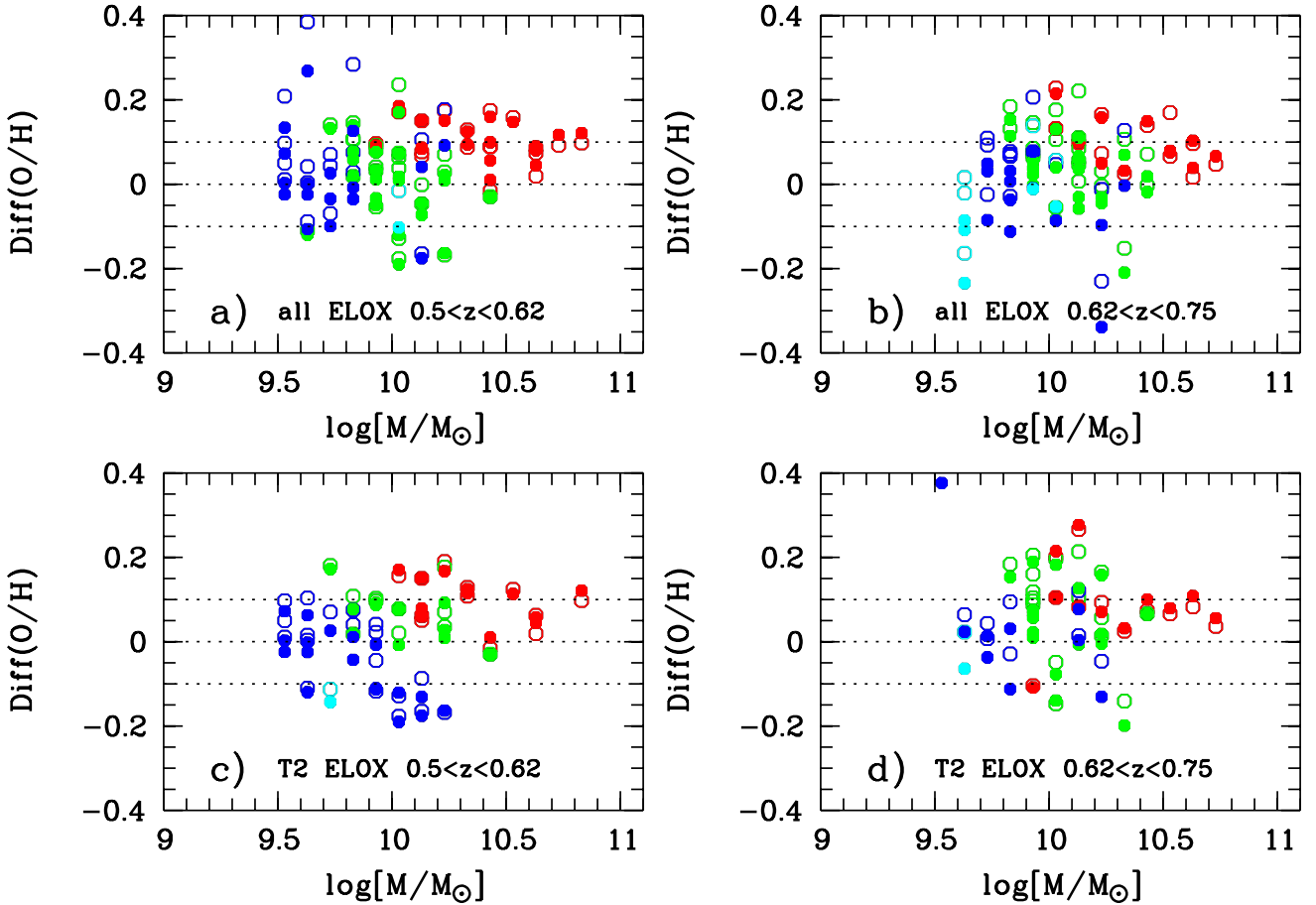
Fig. 7. Difference between the mean O/H at the position of grid points (color-coded as in Fig. 4) and the expected O/H from the formulations of Li13 (open circles) and M10 (filled circles). ELOX galaxies at 0.5 < z < 0.62 are shown in panels a) and c), and at 0.62 < z < 0.75 in panels b) and d), with the lower panels showing only galaxies with T2 (disk) morphologies. Because typical O/H uncertainties are 0.1–0.2 dex, the agreement between the measured and expected O/Hs is quite good, especially in panel c).
