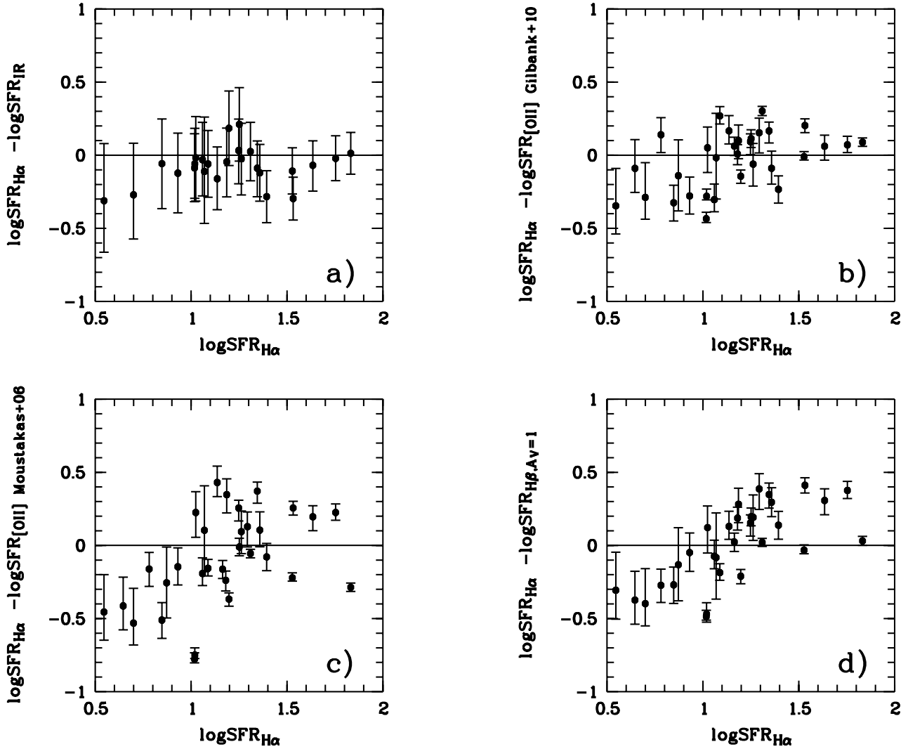
Fig. 2. Comparison of SFRs computed using different methods for zCOSMOS galaxies with ISAAC NIR spectroscopy. Panel a) shows a good agreement (within the measurements errors) of the SFRs from ISAAC H\alpha and SFRs from infrared COSMOS IRAC and MIPS data for the objects with infrared detections (Le Floch et al., in prep.). Panels b)–d) show the comparison of H\alpha -based SFRs with b) SFRs from the [OII] luminosity, applying the calibration reported by Gilbank et al. (2010), their Eq. (8), and taking into account the erratum of Gilbank et al. (2011) of that paper; c) SFRs derived from the [OII] luminosity using Eq. (2) of Maier et al. (2009), based on the study of Moustakas et al. (2006); and d) SFRs from the H\beta luminosity, assuming A_V = 1 (an assumption often used in literature when the Balmer decrement cannot be measured) to derive H\alpha luminosities. The best agreement between the reliable extinction-corrected H\alpha -based SFRs and SFRs estimators based on other ELs (panels b)–d) ) is depicted in panel b) .
