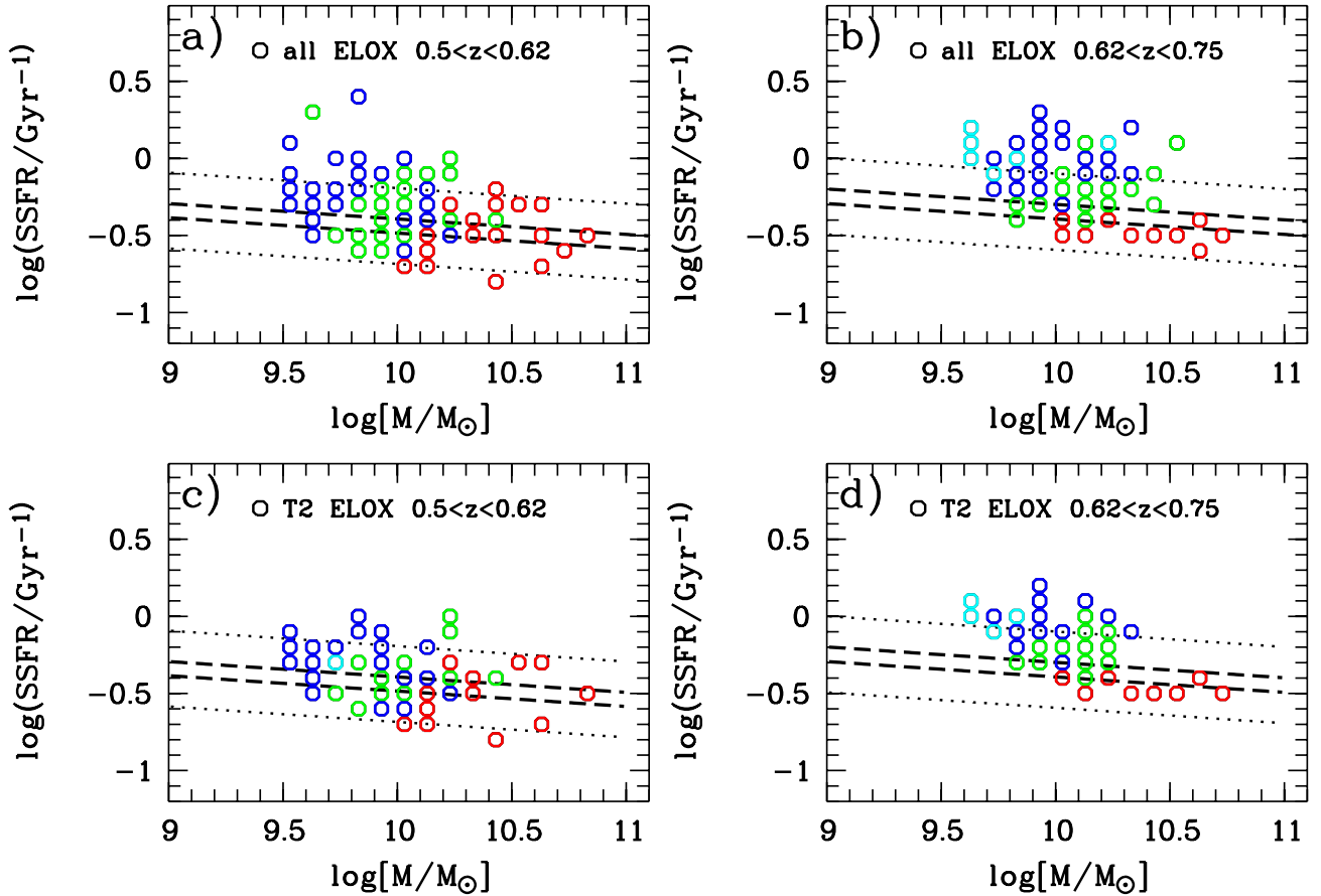
Fig. 6. SSFR-mass relation for the ELOX galaxies at 0.5 < z < 0.62 (panels a) and c)) and at 0.62 < z < 0.75 (panels b) and d)), with the lower panels showing only galaxies with T2 (disk) morphologies. Open circles depict the mean (color-coded as in Fig. 4) metallicity data of ELOX galaxies at the position of grid points with at least three ELOX galaxies within \pm 0.05 dex in \log SFR and \log M from the SSFR and mass values of the respective grid point. It seems that the SFR is a second parameter in the MZR of the zCOSMOS sample at 0.5 < z < 0.75 , because galaxies with higher (S)SFRs generally also have lower metallicities.
