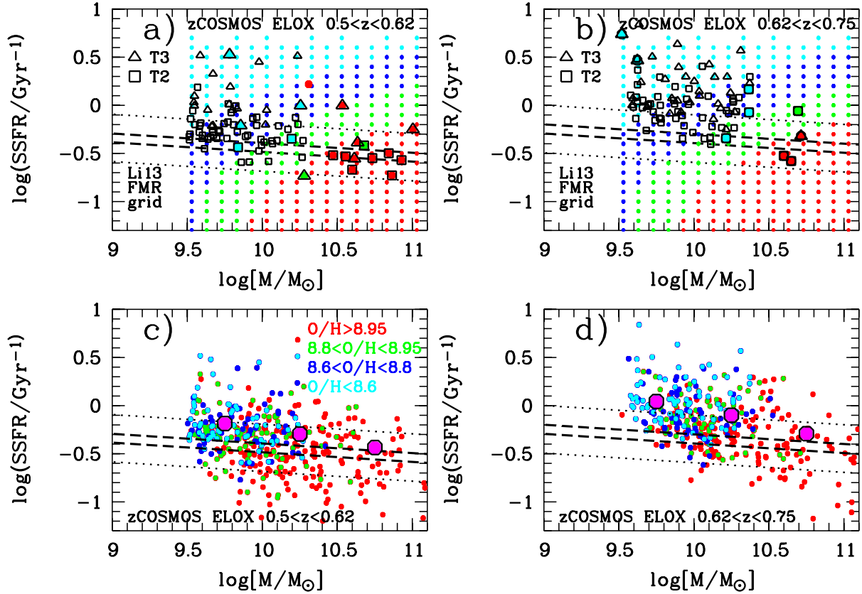
Fig. 4. SSFR-mass relation for zCOSMOS galaxies at 0.5 < z < 0.62 (panels a) and c) and at 0.62 < z < 0.75 (panels b) and d)), with the data points color-coded according to the measured metallicity value (legend in panel c)). The colors of the grid points in panel a) and b) indicate the metallicities expected for the Z(M, \text{SFR}) extrapolation of Li13. In panels a) and b), galaxies with ISAAC spectroscopy are shown as colored symbols, while ELOX galaxies with O/H < 8.6 (the respective cyan circles in panels c) and d)) are shown as black symbols as squares (triangles) for T2 (T3) morphologies. In panels c) and d) the large magenta filled circles show the mean values of the SSFRs in three mass bins. ELOX galaxies with lower R_{23} branch KD02 metallicities, O/H < 8.6 , have typically lower masses ( 9.5 < \log(M/M_{\odot}) < 10.3 ), and preferentially irregular morphologies when they have higher SSFRs. This diagram also indicates that SFR is a second parameter in the MZR of the zCOSMOS sample at 0.5 < z < 0.75 , because galaxies with higher (S)SFRs generally also have lower metallicities.
