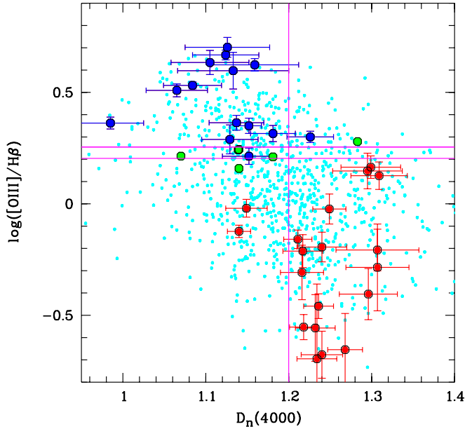
Fig. 3. D_{4000} vs. [\text{O III}] \lambda 5007/\text{H}\beta diagram used to break the R_{23} degeneracy for the 0.5 < z < 0.9 zCOSMOS galaxies (cyan points) without NIR spectroscopy. The 39 zCOSMOS galaxies with ISAAC spectroscopy are shown as blue filled circles for galaxies with low (branch) O/H measurements, red filled circles for galaxies with high (branch) O/H measurements, and green filled circles for the six galaxies with double-valued solutions (note that the D_{4000} and [\text{O III}] \lambda 5007/\text{H}\beta values of two galaxies are almost identical, i.e., the respective green circles coincide). This diagram can be used to break the lower/upper branch R_{23} degeneracy of other 0.5 < z < 0.9 galaxies without NIR spectroscopy, but similar D_{4000} and [\text{O III}] \lambda 5007/\text{H}\beta as the 33 benchmark galaxies with ISAAC spectroscopy and reliable metallicities.
