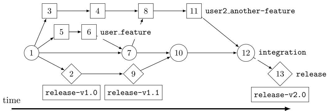
FIGURE 1. The HPCSSS Gitflow . Each circle, square or diamond represents a commit and numbers a possible ordering. An arrow from a commit to another means that the first one is a parent of the second. Text in bold represent branches with commits that were made in this branch in the same horizontal line. Rectangles on the bottom of the figure represent tags.
