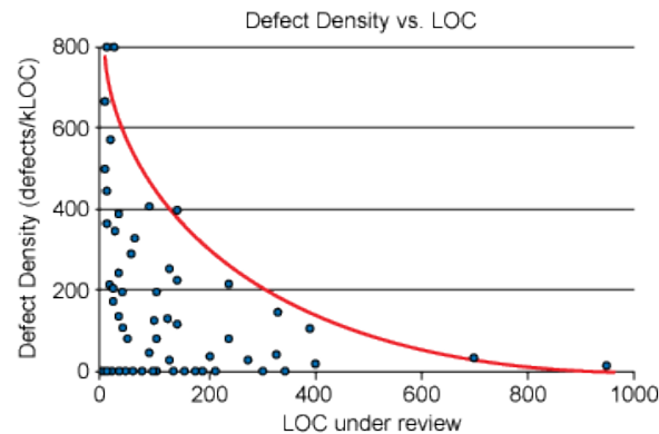
FIGURE 2. As the amount of code under review increases reviewers become less effective at finding defects assuming a constant true number of defects per line of code, extract from The Best Kept Secrets of Peer Code Review [6]
