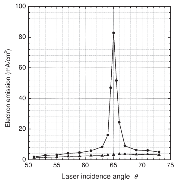
FIG. 2. Photoelectron emission versus incidence angle \theta for p -polarized ( \bullet ) and s -polarized ( \blacktriangle ) laser pulses (at 50 fs and for I = 1 GW/cm 2 ).
