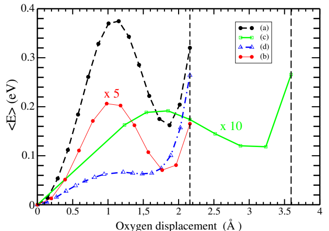
FIG. 2: Average total Energy per atom in eV as a function of oxygen displacement in (Å) for the several cases of oxygen motion : (a) small unit cell; (b) large unit cell and only one oxygen is allowed to move; (c) large unit cell, V vacancy; (d) small unit cell, V on top of Mg. Cases (b) and (c) are amplified 5 and 10 times respectively. All the cases are performed within the LDA approximation. The origin of the displacement corresponds to the position of the last MgO layer, the dashed line at 2.16 Å refers to the first vanadium layer and the dashed line at 3.593 Å to the second one.
