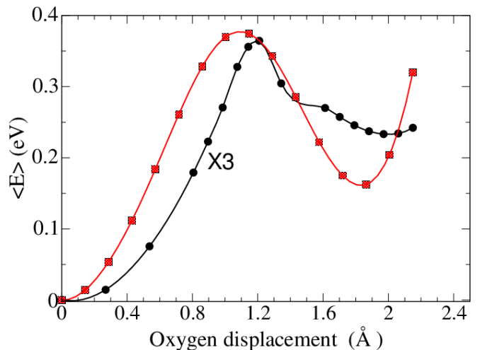
FIG. 3: Calculated average total Energy per atom in eV as a function of oxygen displacement in (Å) with total atomic relaxation (black dots) compared to the unrelaxed structure (red dots). Notice that the atomic relaxation reduces drastically the energy barrier height.
