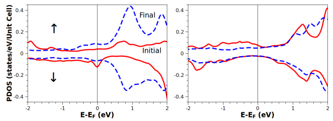
FIG. 5: d_{3z^2-r^2} component of the PDOS for the vanadium atom in front of the moving oxygen (figure 1): V_1 for V on top of O (left panel) and V_2 for V on top of Mg (right panel). The Fermi level is at the zero of energy.
