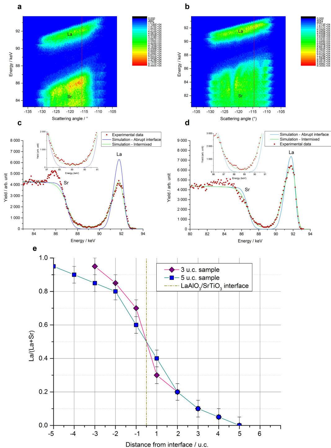
Figure 4. MEIS data in random mode. Incident particles : 100 keV \text{He}^+ ions. (a,b) MEIS random maps ( E_i, \theta_{sc}, N ) of the samples with a film thicknesses of (a) 3 u.c. (b) 5 u.c. Top (-bottom) layers of highest (-lowest) energies correspond to \text{He}^+ particles backscattered on La (-Sr) respectively. Red lines locate the position (at a fixed scattering angle) of the profiles extracted. (c,d) Random MEIS experimental and simulated spectra of the (c) 3 u.c. sample with a backscattering angle of 115,4° (d) 5 u.c. sample with a backscattering angle of 114,5°. The blue curves simulate MEIS theoretical spectra for non-intermixed and fully stoichiometric LAO/STO heterostructures. Experimental spectra are plotted with red dots, whereas the best simulated hetero-structures are represented by a green curve. (e) \text{La}/(\text{La}+\text{Sr}) profile throughout the first atomic layers. The x coordinates locate the cations by the number of unit cells to the interface (+1 = first u.c. in STO, -1 = first u.c. in LAO ...). The film contains a cumulative amount of 0.9 \pm 0.05 Sr in the 5 u.c. sample (thus 4.1 \pm 0.05 La) and 0.5 \pm 0.05 Sr in the 3 u.c. one (thus 2.5 \pm 0.05 La). The La counter-diffusion depths were similar for the two samples, with 0.8 La for 5 u.c., and 0.7 La for 3 u.c. films.
