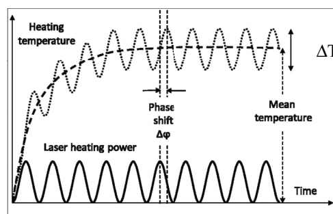
Fig. 1. Phase shift of heating temperature.
