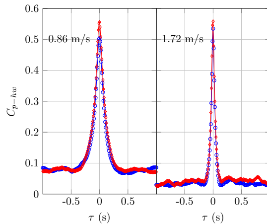
Figure 2. Inter-correlation coefficient of a Pitot tube and a hot-wire signals obtained in He I (red diamonds) and He II (blue circles). Acquisitions performed in HeJet experiment [1]
