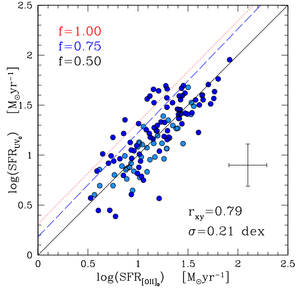
Fig. 17. SFR_{UV_0} vs. SFR_{[OII]_0} corrected for dust extinction using, respectively, \beta_{\text{phot}} and Eq. (11), and EW_{[OII]} and Eq. (14) assuming a Calzetti et al. (2000) law and f = 0.50 . The black line is the 1-to-1 relation that corresponds also to a linear fit to the points. Blue and red lines show the fits with other two different assumptions of f . Blue points are IR-detected galaxies, while light blue points are galaxies with no IR detection.
