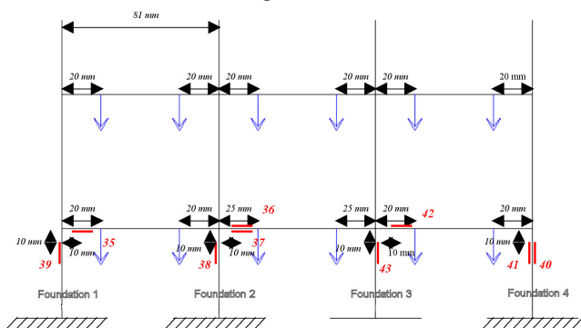
Fig. n°2 : The building model.
