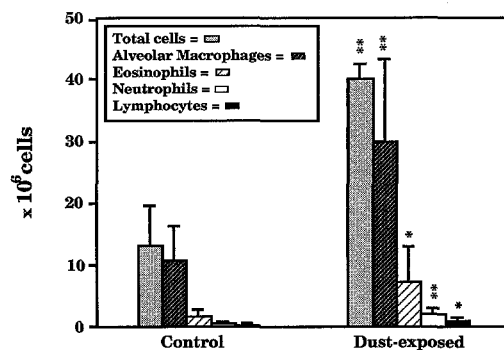
FIGURE 1. Total cell count in bronchoalveolar lavage fluid from control ( n = 6 ) and dust-exposed ( n = 13 ) guinea pigs. The results are expressed as means \pm SD. (*) Difference between dust-exposed and control animals is significant, p < 0.05 ; (**) difference between dust-exposed and control animals is highly significant, p < 0.005 .
