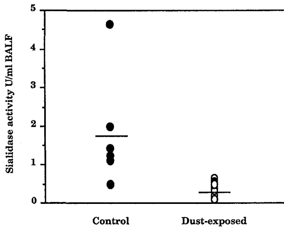
FIGURE 6. Sialidase activity in the cell-free bronchoalveolar lavage fluid (BALF) from control (●) and dust-exposed animals (○). The activity is expressed as enzymatic units per milliliter of concentrated BALF.
