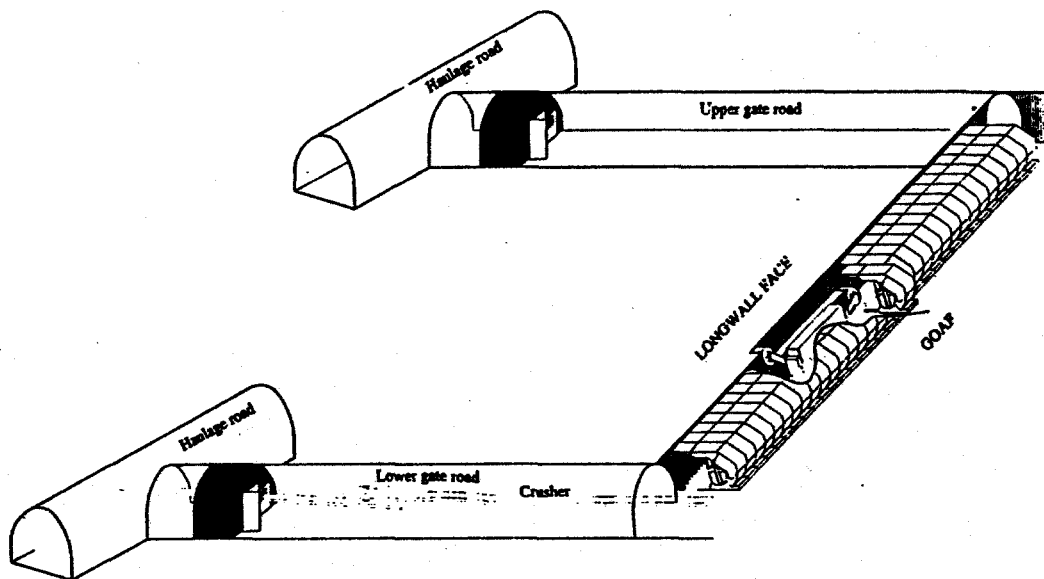
Figure 2: Diagram of a mechanized retreating longwall face
