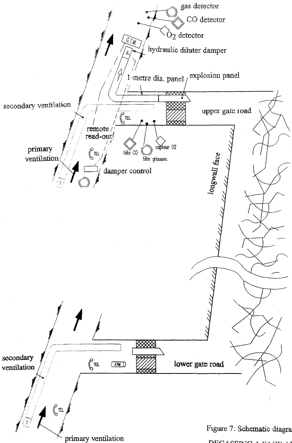
Figure 7: Schematic diagram: degassing a face area.
