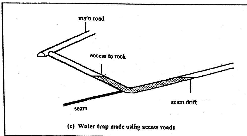
Figure 3: Rapid closure of a district by water trap
