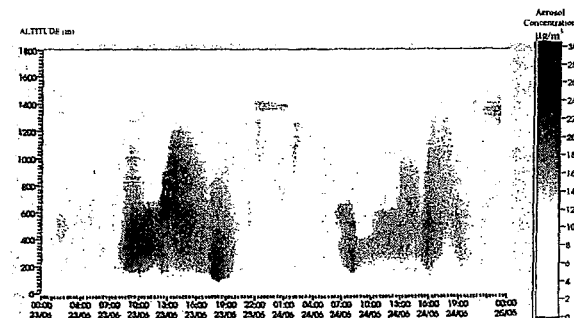
Fig. 3: vertical quantitative aerosols Lidar measurements, temporal evolution.
