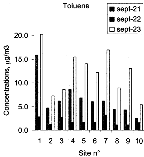
Figure 3 : Toluene concentrations
