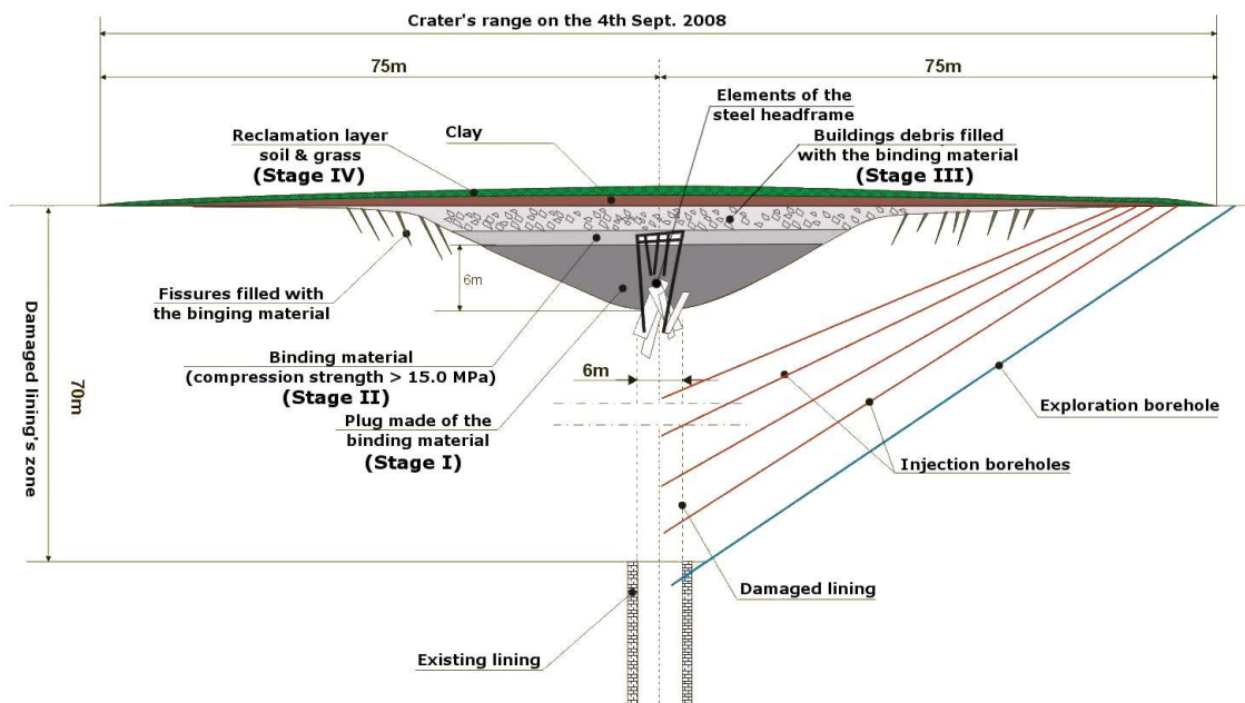
Figure 14 : Schematic illustration of the crater resulting from the catastrophe of shaft V and its fill
