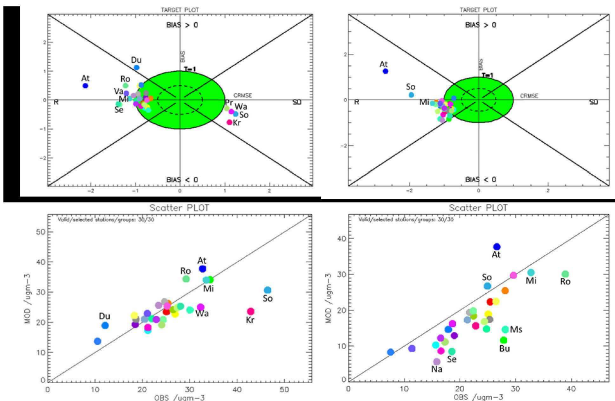
Figure 1: PM10 (left) and NO2 (right) model-observed evaluation. Target diagrams (top) and scatter plots (bottom) provide information for statistics averaged by city areas. For the Target diagrams, stations statistics are sorted and the 10% worst ones are eliminated. The circle on the plot represents the worst remaining statistic. Acronyms are: Du (Dublin), Ro (Rome), Va (Valencia), At (Athens), Mi (Milan), Wa (Warsaw), Kr (Krakow), So (Sofia), Na (Napoli), Ms (Marseille), Se (Sevilla), Pr (Prague). For more information on target diagrams, refer to text.
