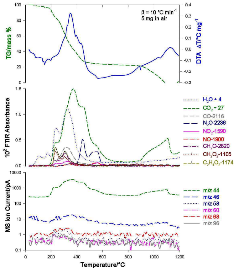
SP1.768: a) TG-DTA; b) FTIR; c) MS results for 5 mg INERIS Smoke Powder 1 heated in air at 10 \text{ °C min}^{-1} .
