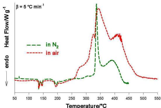
Figure 7 : DSC results for SP1 in air and N 2
