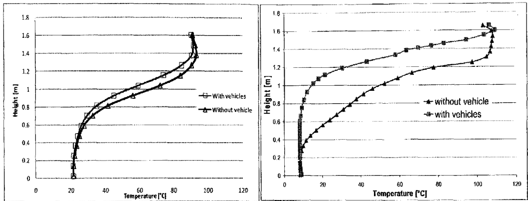
Figure 11: Vertical profile of temperature with and without vehicle obtained with FDS (left) and Phoenics (Right).
