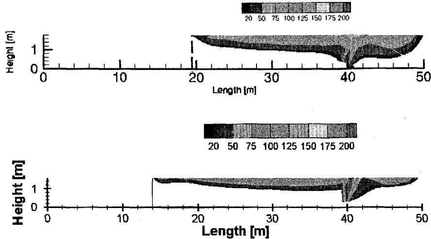
Figure 5: Visualization of the backlayering length obtained with FDS (up) and Phoenics (down).
