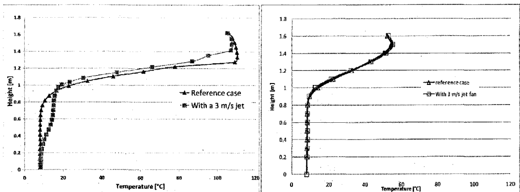
Figure 6: Vertical profile of temperature with and without jet fans at 17 m upstream of the fire obtained with Phoenics (left) and FDS (right).
