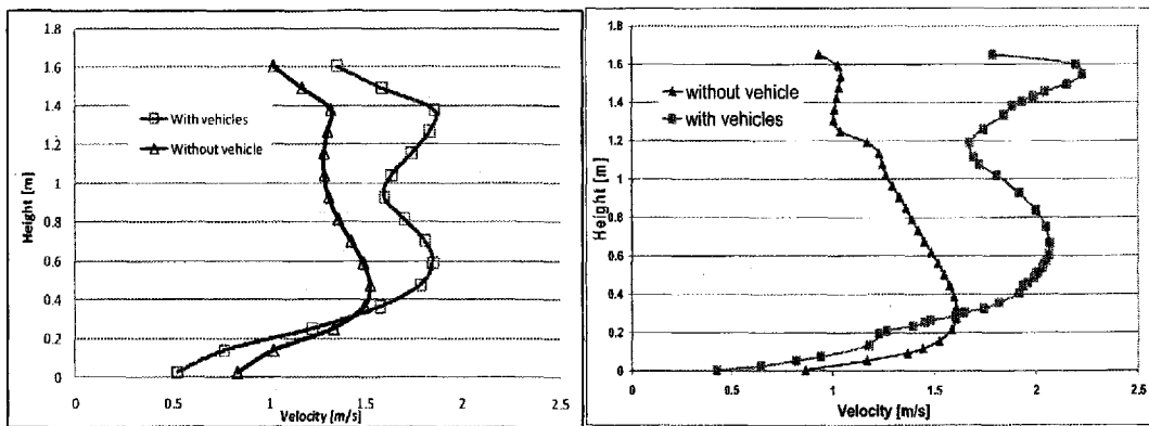
Figure 12: Evolution of the velocity profile in the centerline section, FDS on the left and Phoenics on the right.
