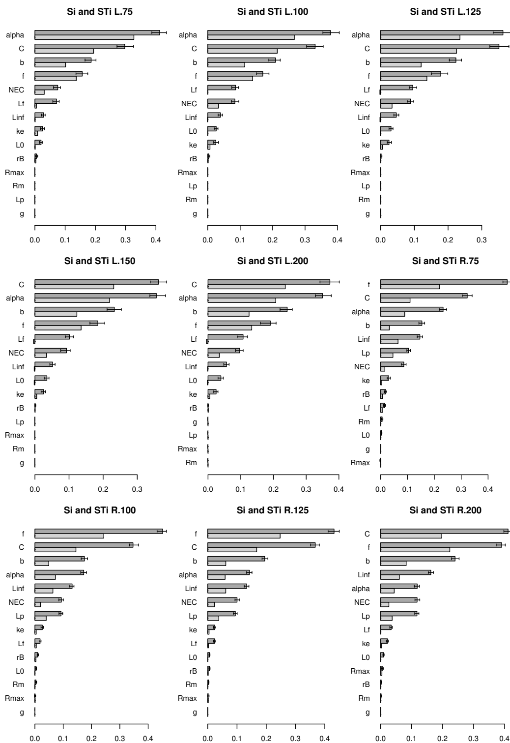
FIGURE C.2 – Sensitivity analysis for the assimilation model (Eq. IX.3). Sensitivity indices at the different times for the growth equation and reproduction equation (e.g. L.75 and R.75 represent respectively sensitivity indices at 75 hours for growth, and reproduction equations). First order indices ( S_i ) are presented in light grey and total order indices ( ST_i ) in dark grey . Parameters were ordered according to the total order Sobol sensitivity indices.
