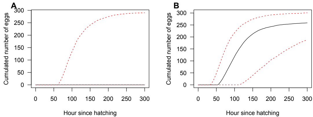
FIGURE C.1 – Uncertainty analysis for reproduction part of the DEBtox the assimilation model for nematode. Panel A represent the uncertainty analysis of the model proposed by Jager et al. (2005) and panel B represent the uncertainty analysis of the model we used (Eq. IX.1). The solid line represent the median of the model output. Dashed lines represent the 95% quantiles of the model output.
