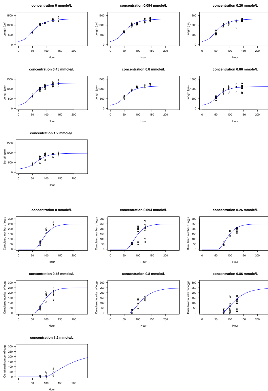
FIGURE D.12 – Model fit for the growth and the reproduction of the generation F2 MGC for each concentration of the toxicity test. Parameters used for the fit correspond to the means of the 1,000 last calculations corresponding to the 1,000 last iterations of the estimation process. The points represent the observed data and the lines represent the model regression curve.
