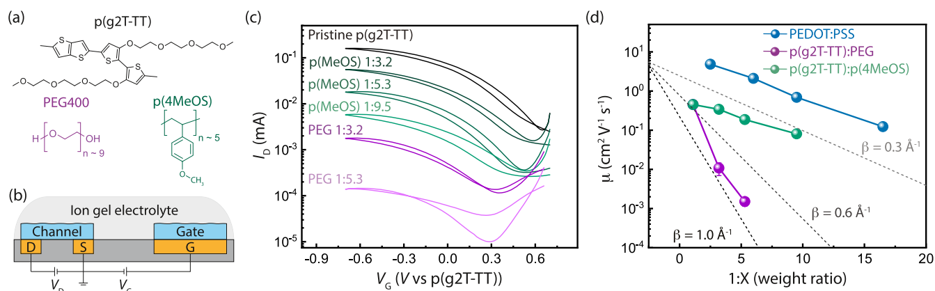
Figure 5. Conductivity scaling for p(g2T-TT):PEG mixed conducting blends. (a) Chemical structures for the semiconducting polymer p(g2T-TT) and blending polymers PEG and p(4MeOS). (b) OEET device test structure using an ion gel electrolyte. (c) OEET transfer characteristics for the diluted p(g2T-TT) blends. (d) Comparison of the mobility scaling PEDOT:PSS (blue), p(g2T-TT):PEG (purple), and p(g2T-TT):p(4MeOS) (green) diluted blends. For reference, the slopes corresponding to tunneling coefficients of \beta = 0.3, 0.6, and 1.0 \text{ \AA}^{-1} are plotted (gray dashed lines). We note that the weight of the pegylated side chains of p(g2T-TT) was considered as a part of the non-conductive weight fraction.
