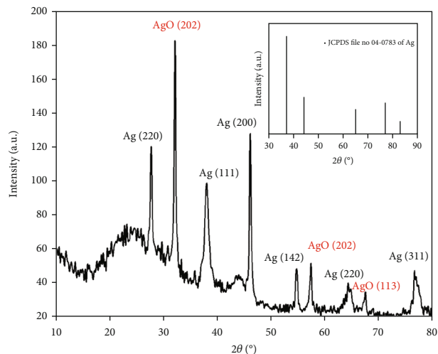
FIGURE 4: XRD pattern of the silver nanoparticles synthesized from aqueous seed extracts of A. pavonina .
