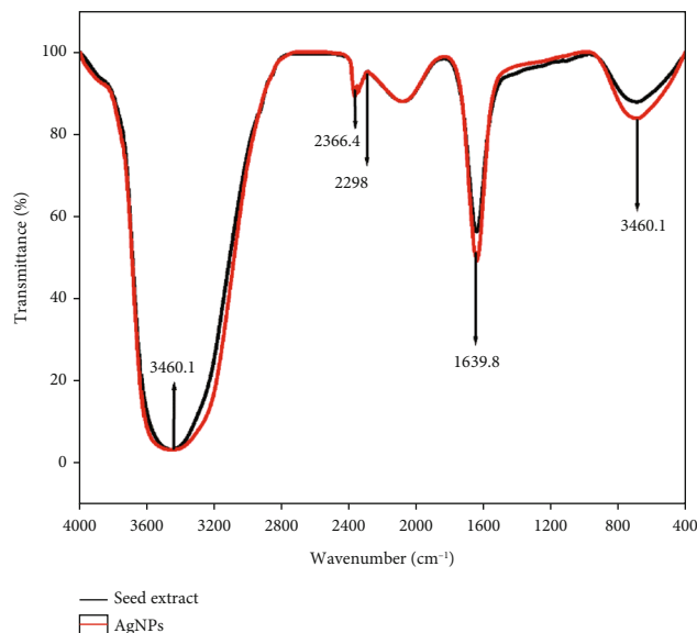
FIGURE 5: FTIR spectra of silver nanoparticles and seed extract.
