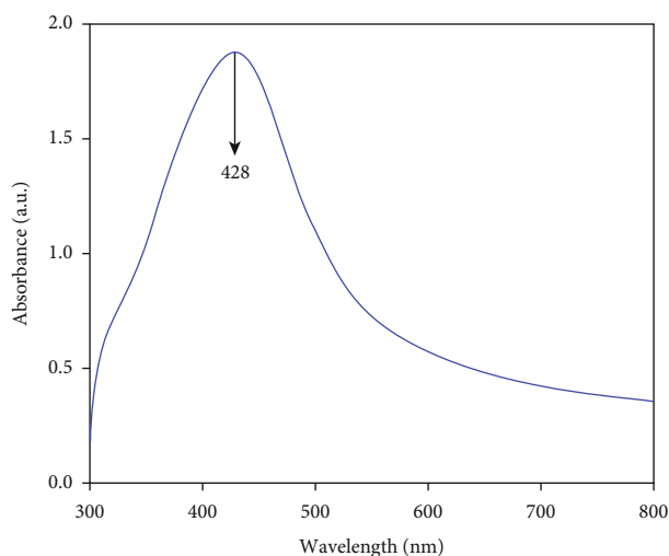
FIGURE 1: UV-visible spectrum of AgO nanoparticles.
