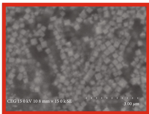
FIGURE 2: SEM image of synthesized silver nanoparticles.
