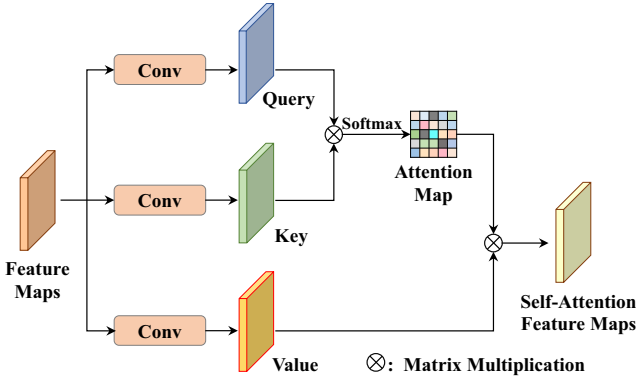
Figure 1: The structure of standard self-attention mechanism.
