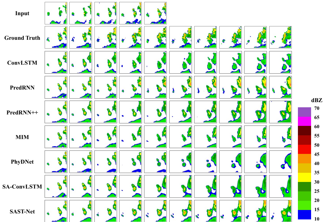
Figure 8: The prediction results of all models on CIKM 2017 dataset. The 5 images in the first line are the input, and the second line is the real value. The other rows are the predictions of various models.
