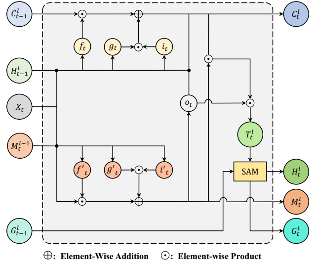
Figure 3: The structure of SAST-LSTM cell.
