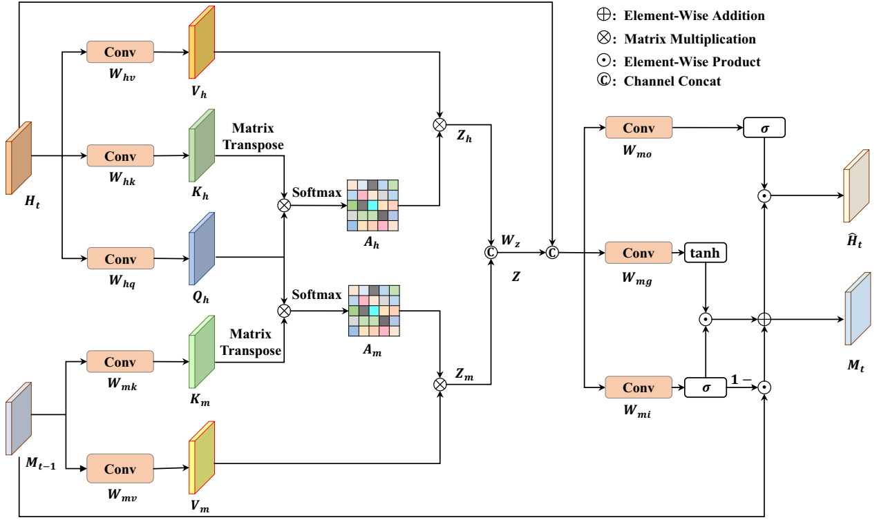
Figure 2: The structure of self-attention memory module (SAM).
