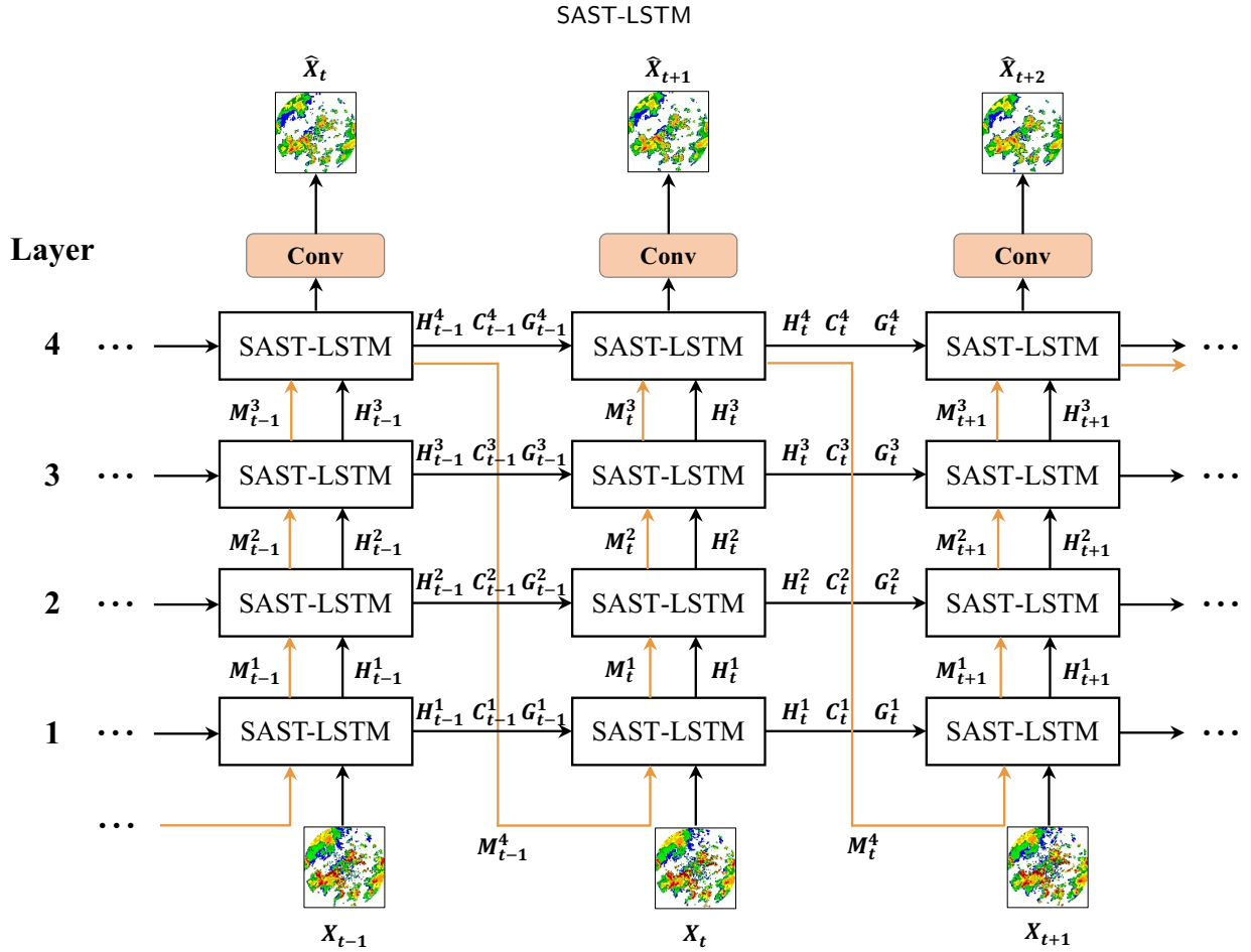
Figure 4: The overall architecture of SAST-Net built by stacking SAST-LSTM cell.
