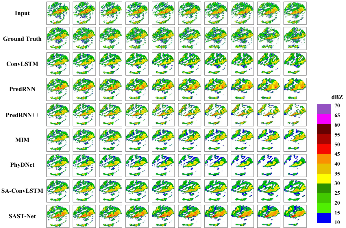
Figure 7: The prediction results of all models on Guangzhou Station dataset. The 10 images in the first row are the input, and the 10 images in the second row are the real values. The other rows are the predictions of various models.
