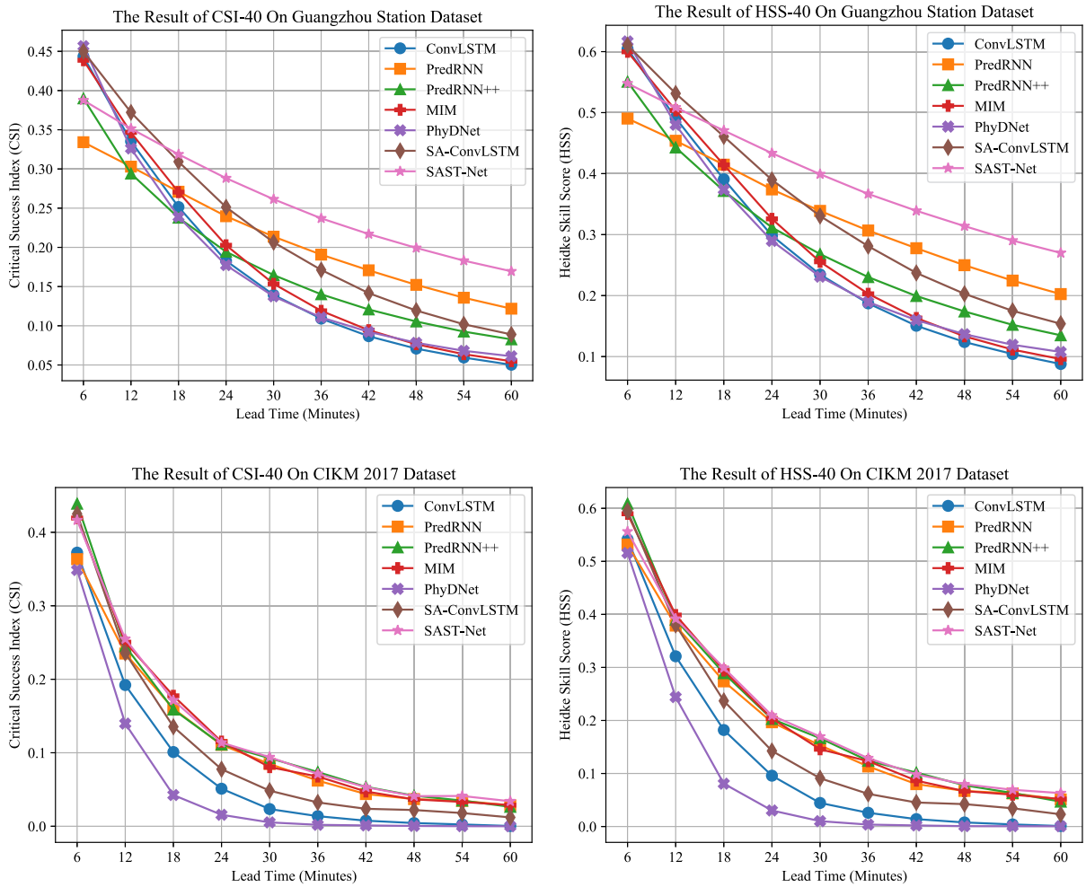
Figure 6: The frame-by-frame variation curves of different models in terms of CSI and HSS scores on Guangzhou Station and CIKM 2017 datasets when threshold \tau = 40 .
