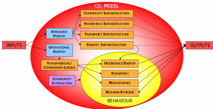
Figure 9: Christie Walk CO 2 model conceptualisation
