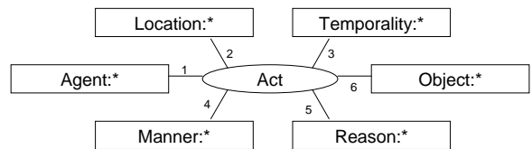
Figure 5. Representation, in the form of a semantic network, of an action conducted by an Agent on an Object. Concepts of Agent, Location, Temporality, Manner, Reason and Object are implemented as functional groups, as well as the Act relationship.
