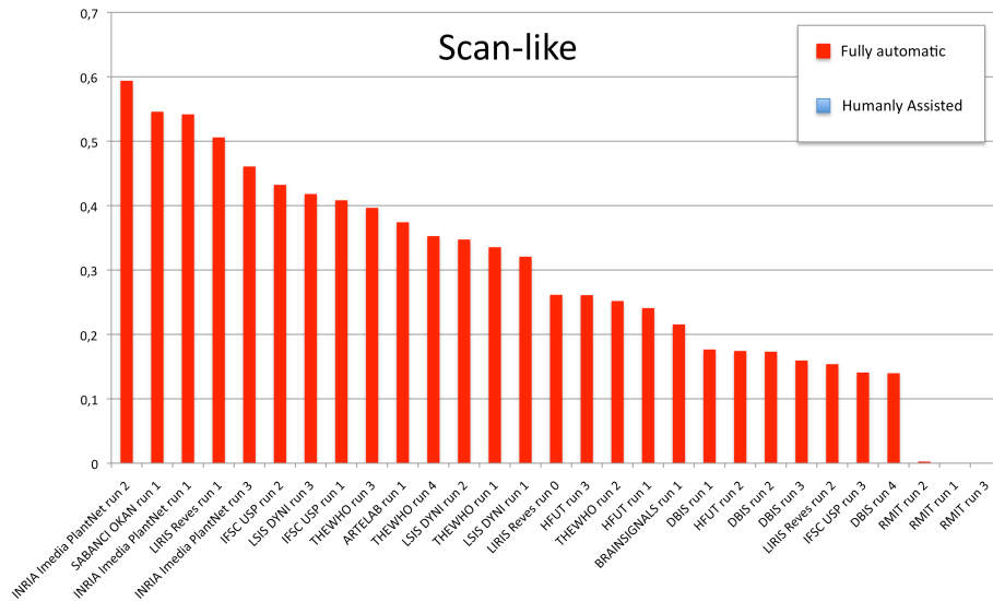
Fig. 15. Scores for Scan-like images
