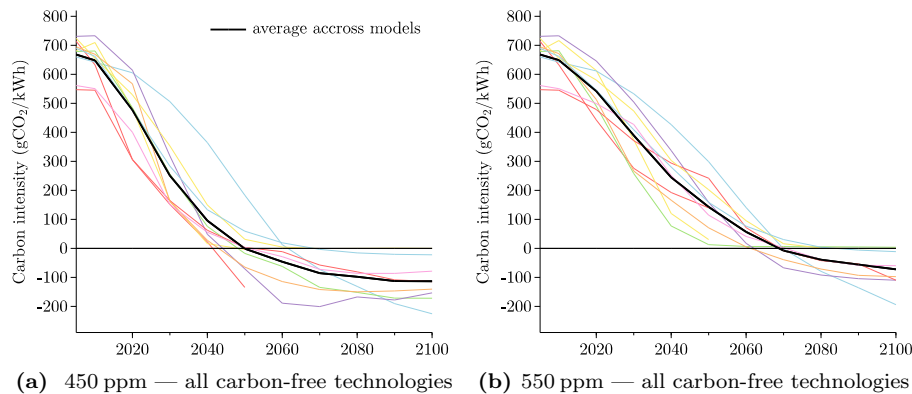
Figure 1: Carbon content of electricity at the global scale in two scenarios: (a) stringent GHG concentration target (consistent with 2^{\circ}\text{C} ); (b) less stringent GHG concentration target (consistent with 3^{\circ}\text{C} ). Each thin line corresponds to the pathway simulated by one integrated assessment model (the reported carbon intensity for 2005 and 2010 varies among IAMs because they use different scopes and sources of historical data for calibration). In both cases, bio-energy with carbon capture and storage (BECCS) allows to reduce the carbon content of electricity to below-zero levels by the end of the century.
