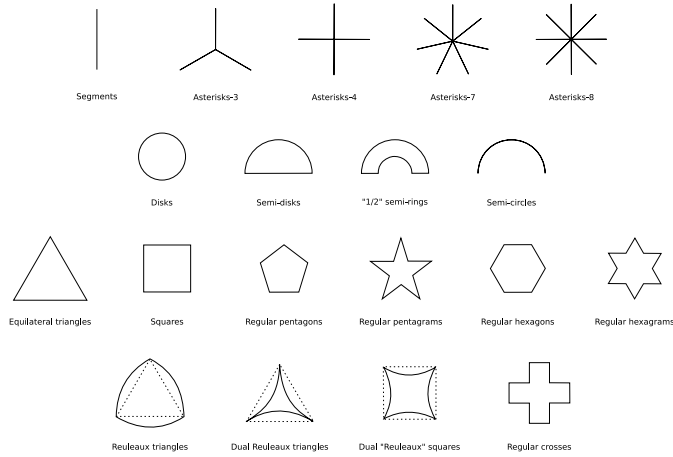
Fig. 2. Family \mathcal{F}_1 of 2D compact sets.
