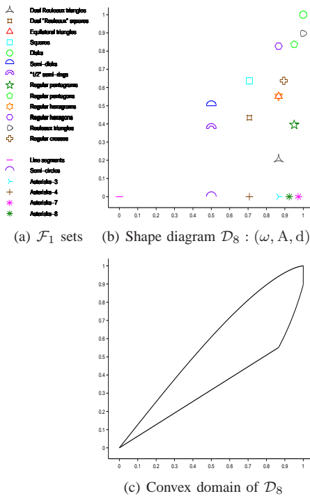
Fig. 3. Shape diagram \mathcal{D}_8 (b) for the compact sets (a) of the family \mathcal{F}_1 with the boundaries of the convex domain (c).
