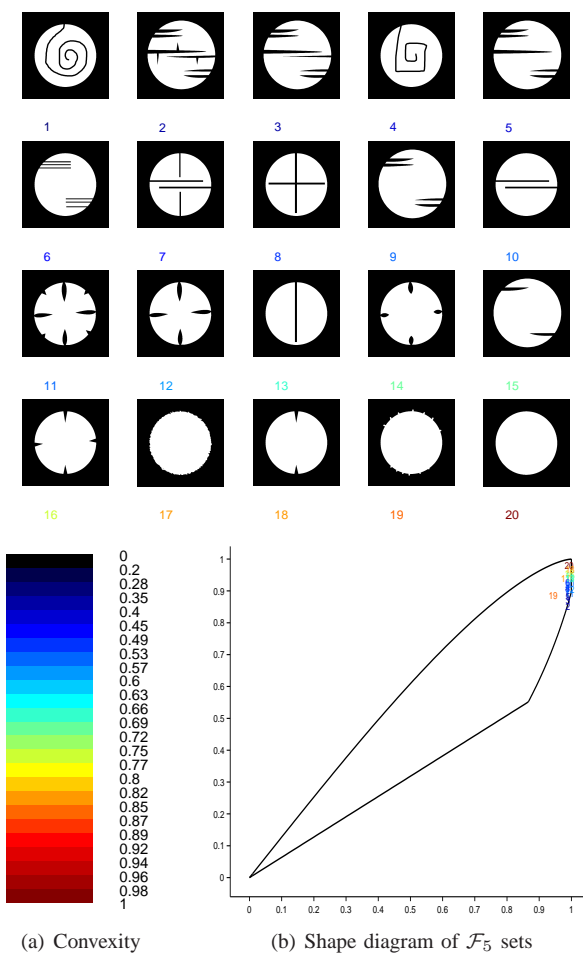
Fig. 6. Family \mathcal{F}_5 of twenty 2D compact sets, represented in white on binary images. All these sets have a 'disk' shape. The color of the number is related to the convexity parameter value (a). Discrimination of similar sets for this family \mathcal{F}_5 (b) mapped onto the shape diagram \mathcal{D}_8 .
