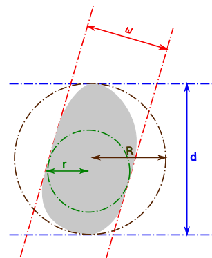
Fig. 1. Geometrical functionals of a compact set: radii of inscribed ( r ) and circumscribed ( R ) circles, minimum ( \omega ) and maximum ( d ) Feret diameters.
