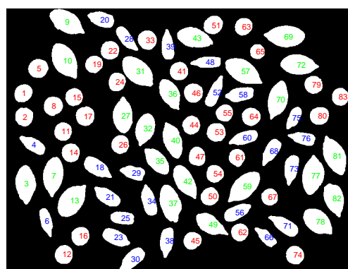
(a) Seeds image
