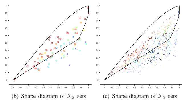
(b) Shape diagram of \mathcal{F}_2 sets
