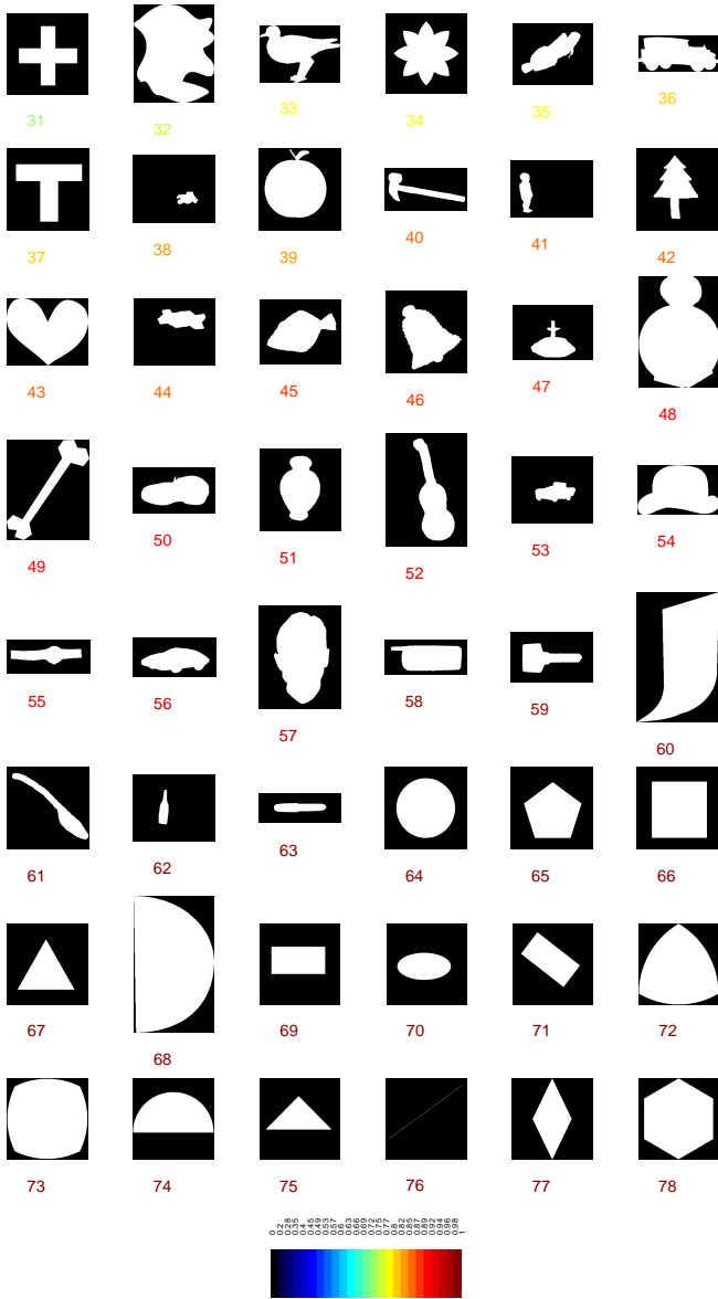
(a) Range of convexity values
