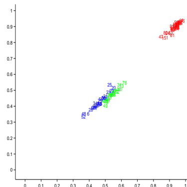
(b) Shape diagram of seeds
