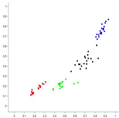
Fig. 8. Discrimination of sets mapped onto the shape diagram \mathcal{D}_8 . The set locations are points whose the color is related to the group to which the set belongs: red for the sets of 'watch' shape, blue for the sets of 'apple' shape, green for the sets of 'sea-snake' shape, and black for the sets of 'camel' shape.
