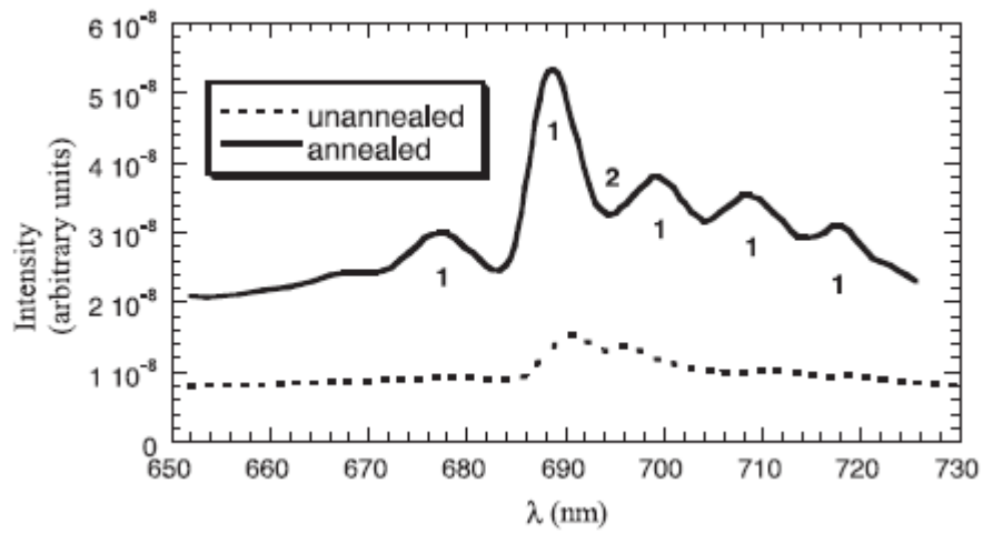
Figure 5: Emission spectra of MgAl_2O_4 obtained at room temperature ( \lambda_{exc}=395\text{ nm} ) before and after neutral annealing.
