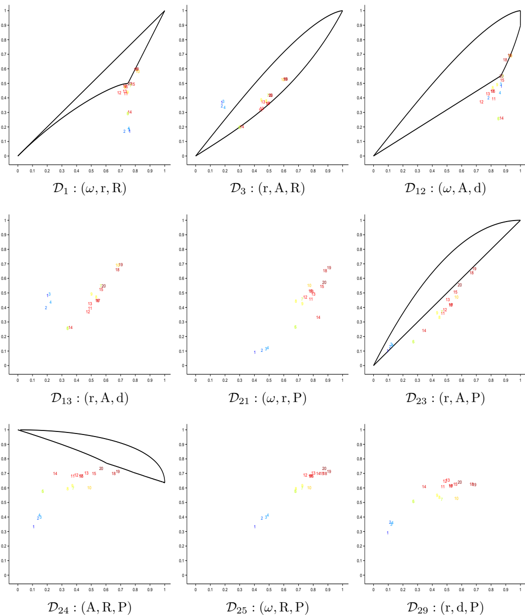
Figure 6.1: Family \mathcal{F}_3^{dsc} of twenty 2D discretized simply connected compact sets with 'triangle' shape, mapped into nine shape diagrams (chosen according to the results synthetized in [9]). The color of the number is related to the convexity parameter value.
