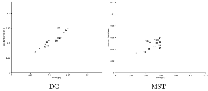
Figure 6.4: Two dispersion quantifications for all shape diagrams applied on the family \mathcal{F}_3^{disc} . For each representation (according to the models DG and MST, respectively), indices k \in \llbracket 1, 29 \rrbracket \setminus (\llbracket 4, 10 \rrbracket \cup \llbracket 14, 20 \rrbracket) of the shape diagrams \mathcal{D}_k is located according to its \mu and \sigma values.
