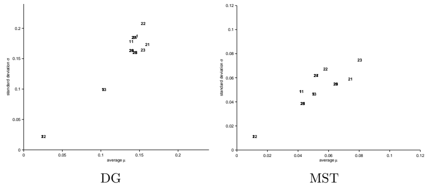
Figure 6.5: Two dispersion quantifications for all shape diagrams applied on the family \mathcal{F}_4^{disc} . For each representation (according to the models DG and MST, respectively), indices k \in \llbracket 1, 29 \rrbracket \setminus (\llbracket 4, 10 \rrbracket \cup \llbracket 14, 20 \rrbracket) of the shape diagrams \mathcal{D}_k is located according to its \mu and \sigma values.
