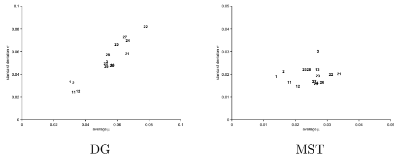
Figure 6.6: Two dispersion quantifications for all shape diagrams applied on the family \mathcal{F}_5^{disc} . For each representation (according to the models DG and MST, respectively), indices k \in \llbracket 1, 29 \rrbracket \setminus (\llbracket 4, 10 \rrbracket \cup \llbracket 14, 20 \rrbracket) of the shape diagrams \mathcal{D}_k is located according to its \mu and \sigma values.
