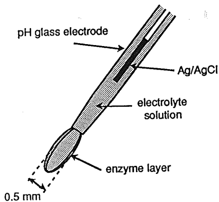
Figure 1. Immersion method used to immobilize enzyme on a micro-pH electrode.
