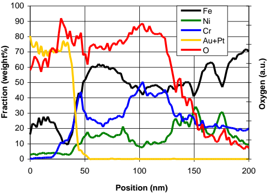
Figure 7 – EDS profile. Site 1A at the surface of specimen 1594-T112-06 (304L).
