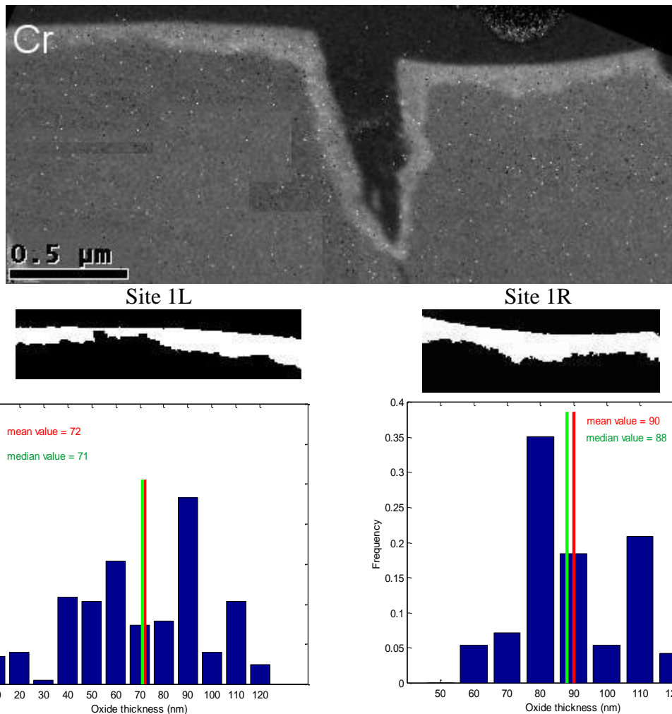
Figure 13 – EFTEM analysis of Cr-rich inner oxide layer at the surface of specimen T217-01 on site 1 (316L)
