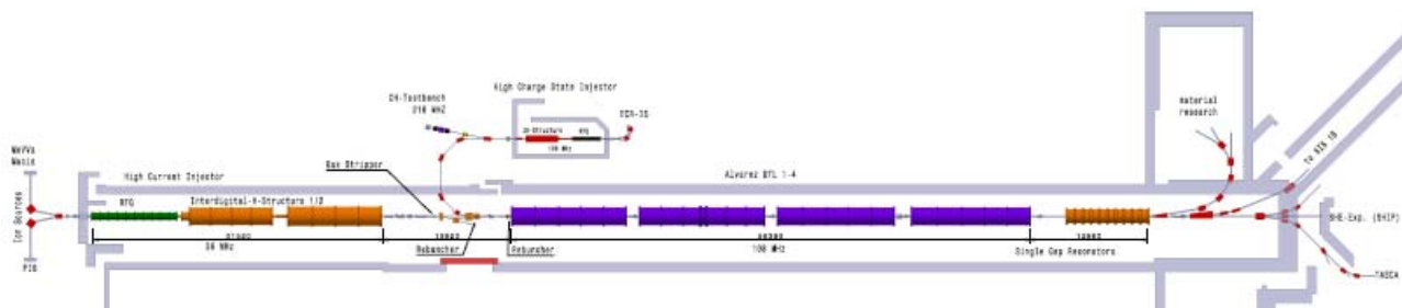
Figure 1: Scheme of the UNILAC accelerator.
