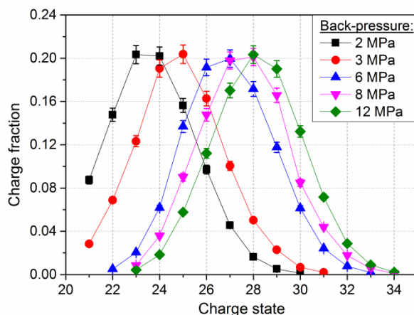
Figure 3: Charge state distribution for U on H_2 with increasing back-pressure on the gas inlet.
