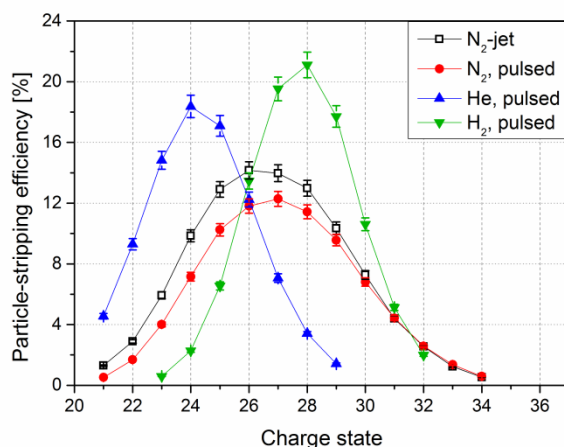
Figure 4: Measured stripping efficiencies for U on H_2 , He and N_2 using the pulsed gas cell (full symbols) and the N_2 -jet (open symbols); all distributions except for H_2 are equilibrated, suggesting that even higher charge states can be populated with H_2 at higher gas densities. Lower efficiencies for pulsed N_2 compared to the N_2 -jet are caused by decreased transmission.
