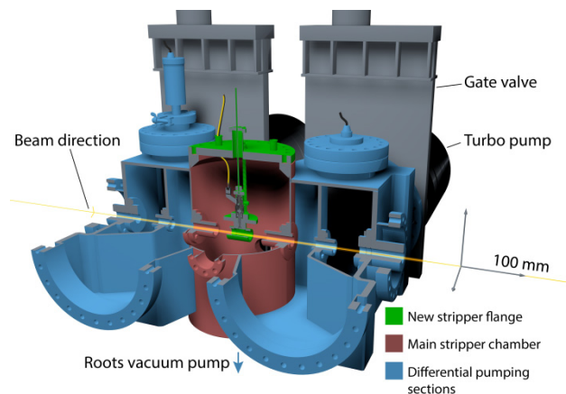
Figure 1: 3D model of the GSI UNILAC gas stripper.
