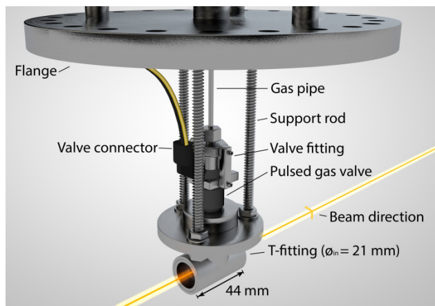
Figure 2: 3D model of the new stripper flange.
